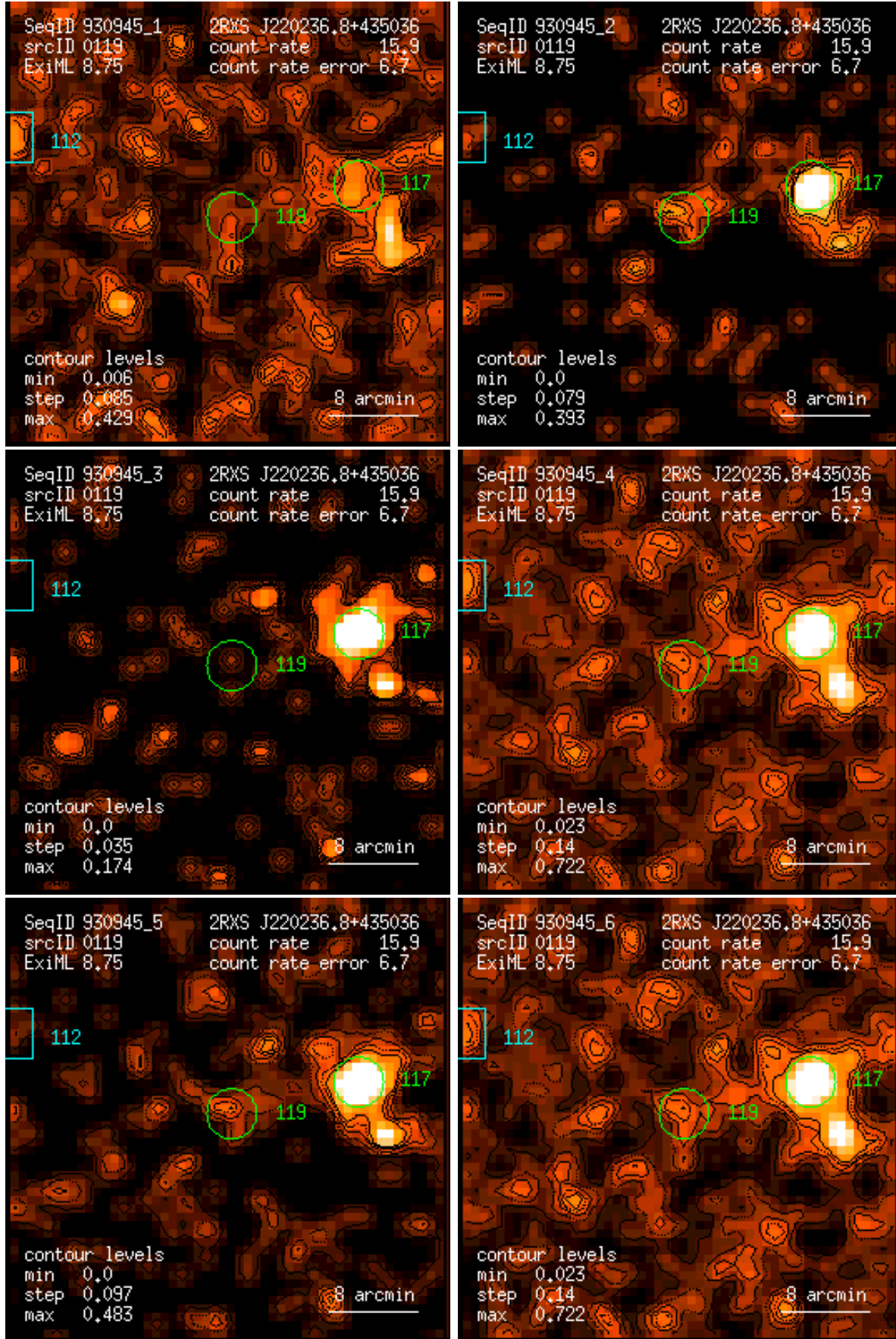
Figure 119: RASS 930945: detection 0119: band rate images, Gaussian filter: (1) PSPC channels 11 – 41, (2) 52 – 90, (3) 91 – 201, (4) 11 – 235, (5) 52 – 201, (6) 11 – 201. Broad band rates in counts/ks. Band rate contour levels in counts/ks/arcmin 2 .
