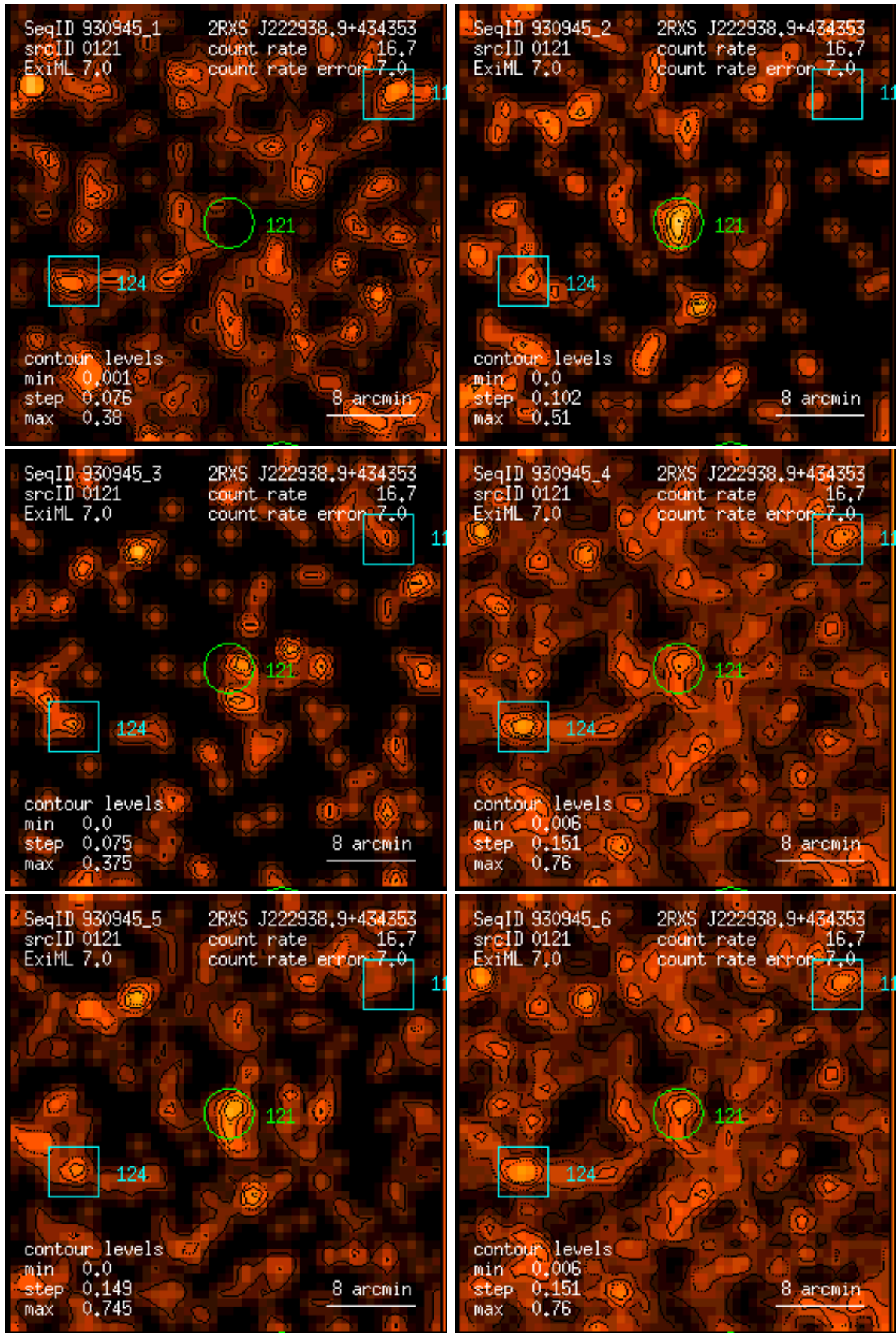
Figure 121: RASS 930945: detection 0121: band rate images, Gaussian filter: (1) PSPC channels 11 – 41, (2) 52 – 90, (3) 91 – 201, (4) 11 – 235, (5) 52 – 201, (6) 11 – 201. Broad band rates in counts/ks. Band rate contour levels in counts/ks/arcmin 2 .
