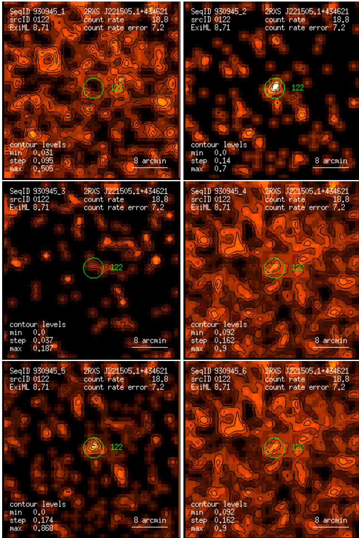
Figure 122: RASS 930945: detection 0122: band rate images, Gaussian filter: (1) PSPC channels 11 – 41, (2) 52 – 90, (3) 91 – 201, (4) 11 – 235, (5) 52 – 201, (6) 11 – 201. Broad band rates in counts/ks. Band rate contour levels in counts/ks/arcmin 2 .
