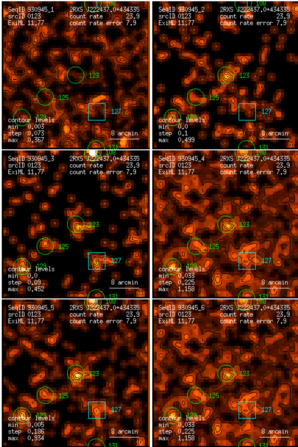
Figure 123: RASS 930945: detection 0123: band rate images, Gaussian filter: (1) PSPC channels 11 – 41, (2) 52 – 90, (3) 91 – 201, (4) 11 – 235, (5) 52 – 201, (6) 11 – 201. Broad band rates in counts/ks. Band rate contour levels in counts/ks/arcmin 2 .
