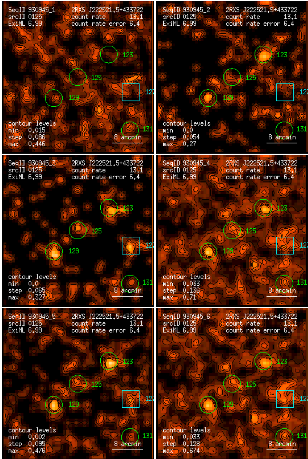
Figure 125: RASS 930945: detection 0125: band rate images, Gaussian filter: (1) PSPC channels 11 – 41, (2) 52 – 90, (3) 91 – 201, (4) 11 – 235, (5) 52 – 201, (6) 11 – 201. Broad band rates in counts/ks. Band rate contour levels in counts/ks/arcmin 2 .
