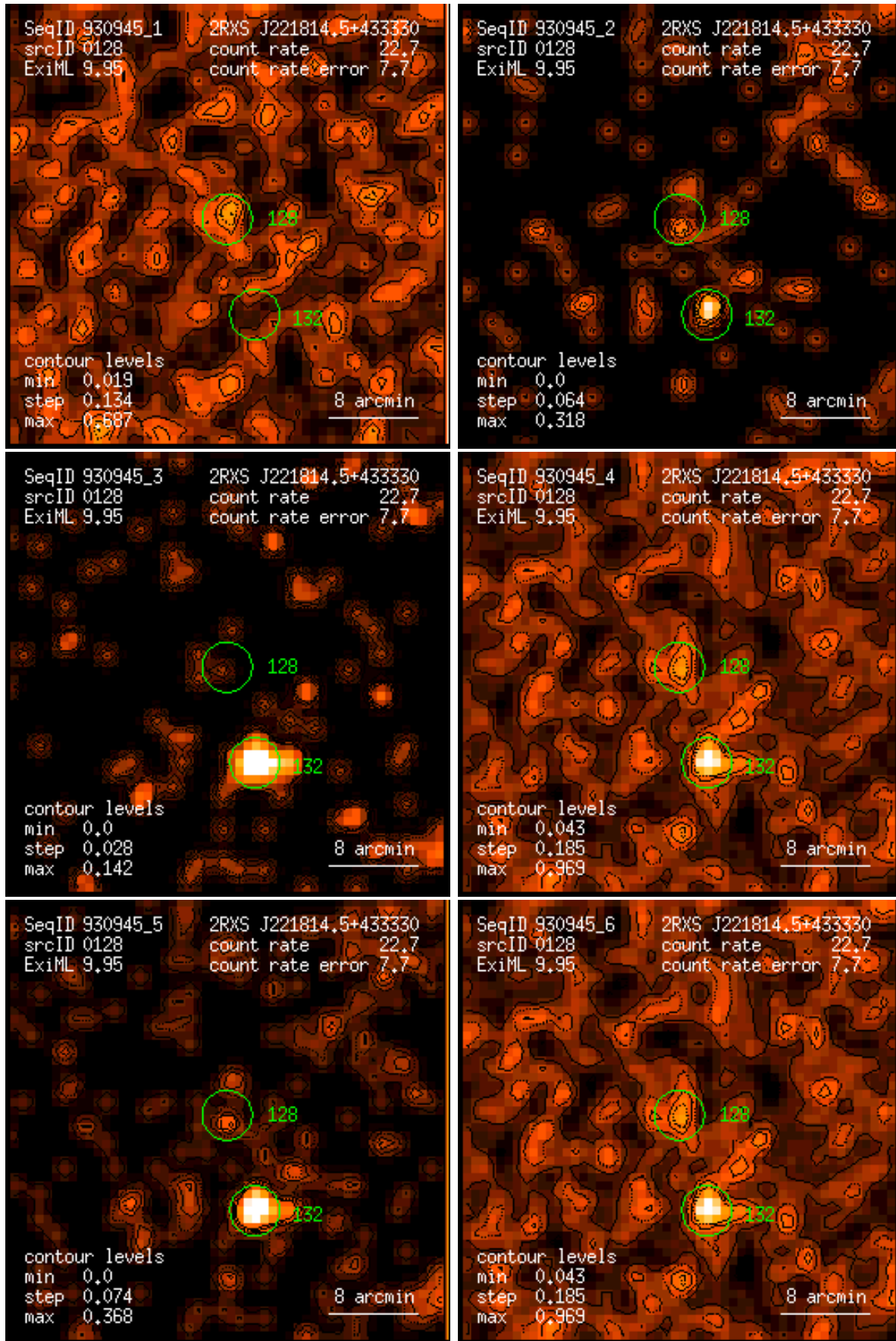
Figure 128: RASS 930945: detection 0128: band rate images, Gaussian filter: (1) PSPC channels 11 – 41, (2) 52 – 90, (3) 91 – 201, (4) 11 – 235, (5) 52 – 201, (6) 11 – 201. Broad band rates in counts/ks. Band rate contour levels in counts/ks/arcmin 2 .
