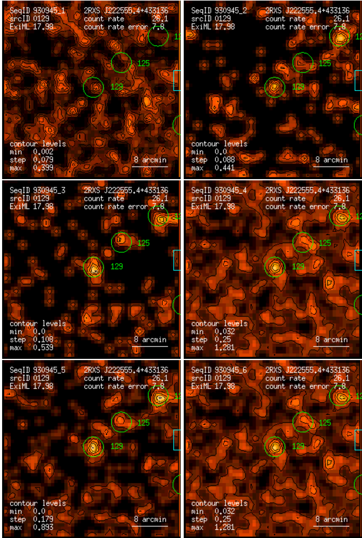
Figure 129: RASS 930945: detection 0129: band rate images, Gaussian filter: (1) PSPC channels 11 – 41, (2) 52 – 90, (3) 91 – 201, (4) 11 – 235, (5) 52 – 201, (6) 11 – 201. Broad band rates in counts/ks. Band rate contour levels in counts/ks/arcmin 2 .
