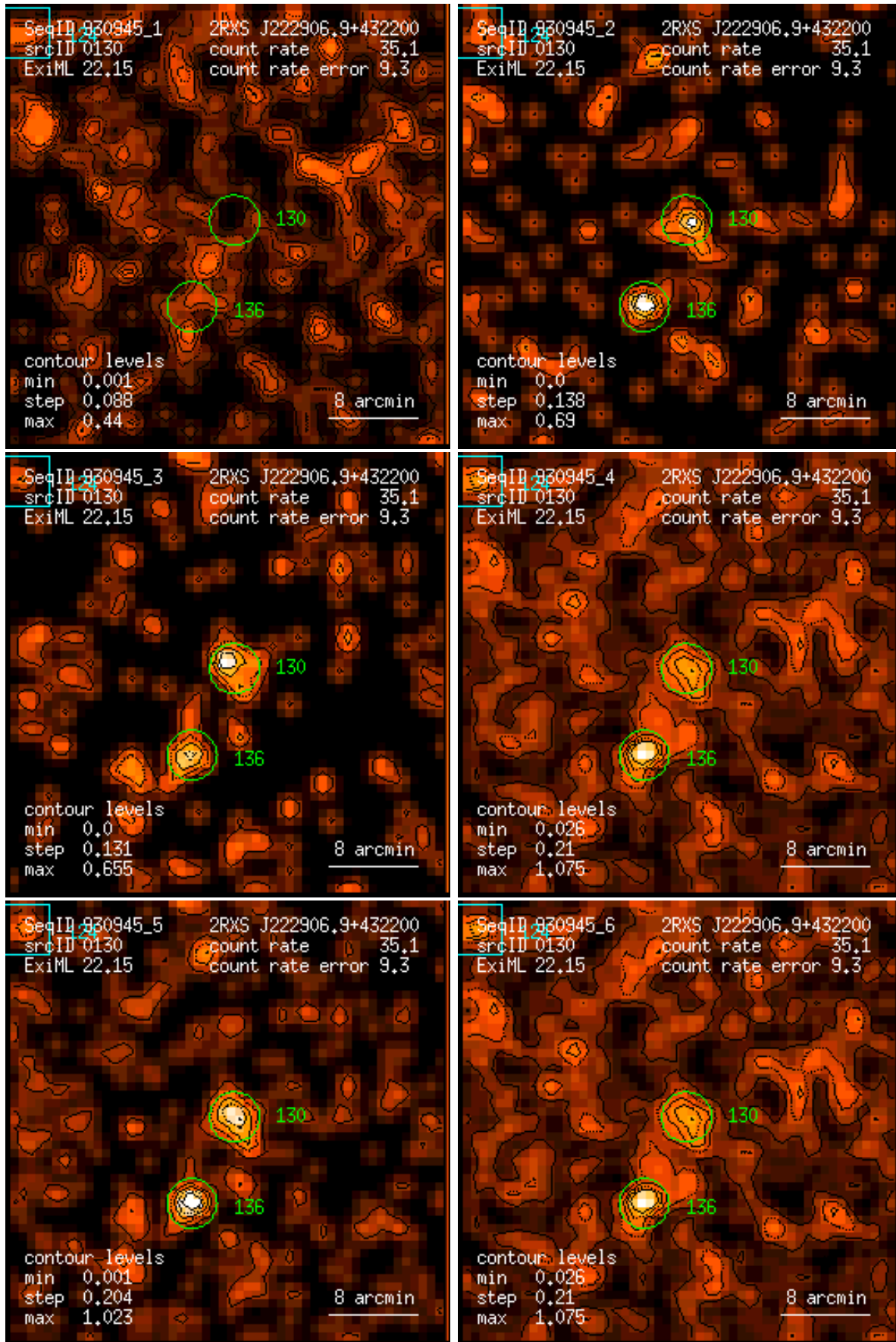
Figure 130: RASS 930945: detection 0130: band rate images, Gaussian filter: (1) PSPC channels 11 – 41, (2) 52 – 90, (3) 91 – 201, (4) 11 – 235, (5) 52 – 201, (6) 11 – 201. Broad band rates in counts/ks. Band rate contour levels in counts/ks/arcmin 2 .
