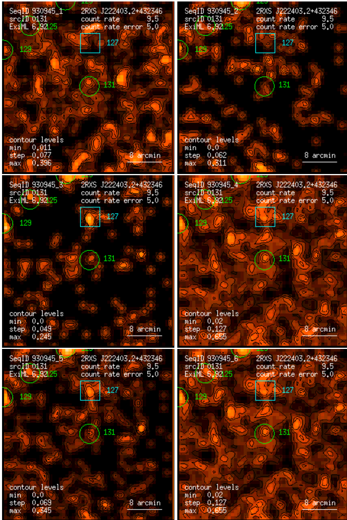
Figure 131: RASS 930945: detection 0131: band rate images, Gaussian filter: (1) PSPC channels 11 – 41, (2) 52 – 90, (3) 91 – 201, (4) 11 – 235, (5) 52 – 201, (6) 11 – 201. Broad band rates in counts/ks. Band rate contour levels in counts/ks/arcmin 2 .
