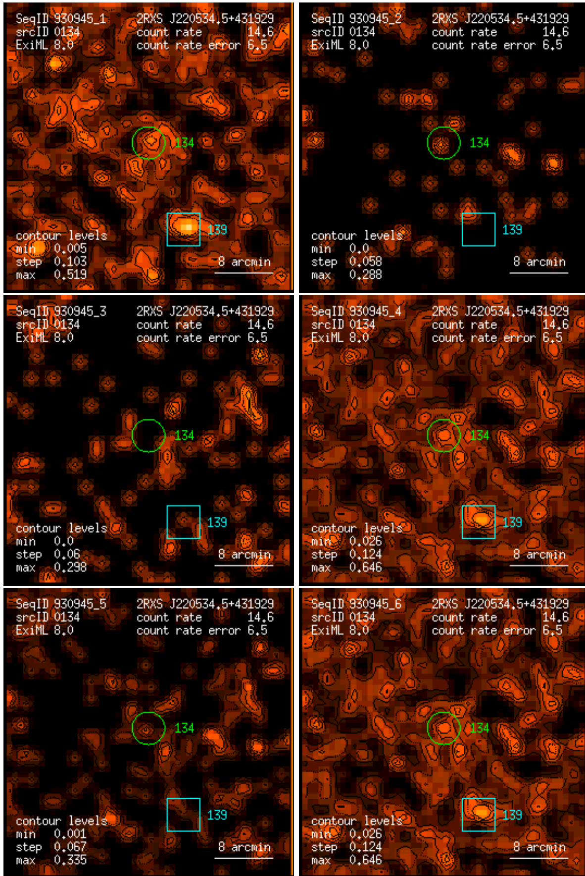
Figure 134: RASS 930945: detection 0134: band rate images, Gaussian filter: (1) PSPC channels 11 – 41, (2) 52 – 90, (3) 91 – 201, (4) 11 – 235, (5) 52 – 201, (6) 11 – 201. Broad band rates in counts/ks. Band rate contour levels in counts/ks/arcmin 2 .
