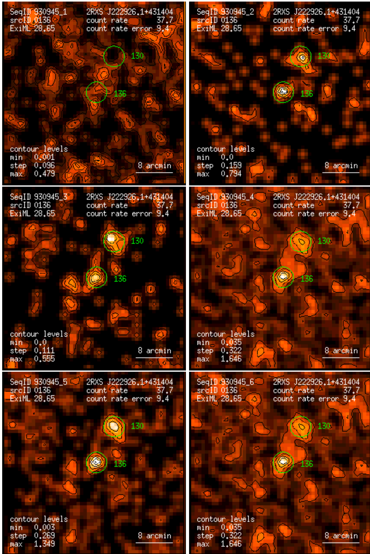
Figure 136: RASS 930945: detection 0136: band rate images, Gaussian filter: (1) PSPC channels 11 – 41, (2) 52 – 90, (3) 91 – 201, (4) 11 – 235, (5) 52 – 201, (6) 11 – 201. Broad band rates in counts/ks. Band rate contour levels in counts/ks/arcmin 2 .
