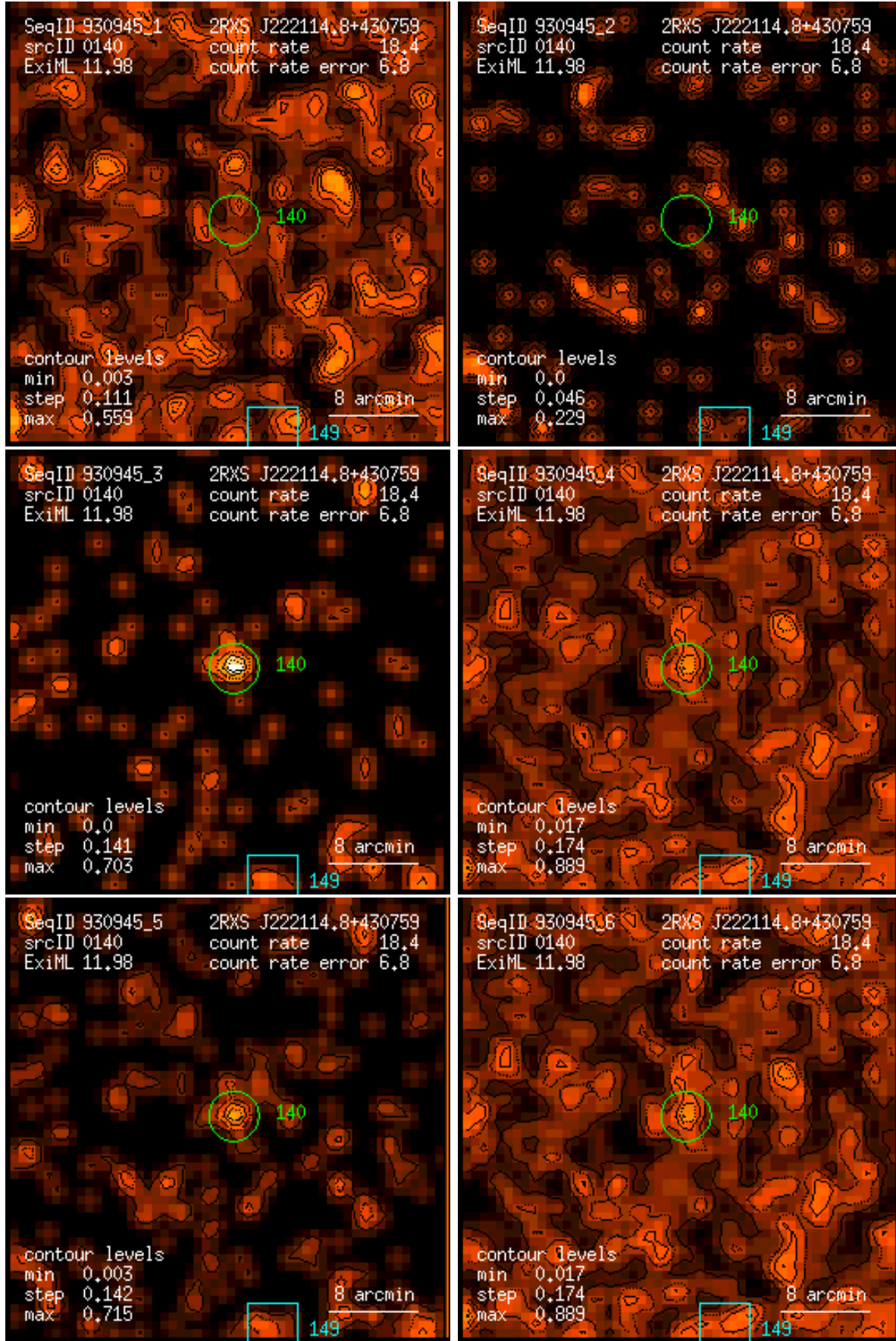
Figure 140: RASS 930945: detection 0140: band rate images, Gaussian filter: (1) PSPC channels 11 – 41, (2) 52 – 90, (3) 91 – 201, (4) 11 – 235, (5) 52 – 201, (6) 11 – 201. Broad band rates in counts/ks. Band rate contour levels in counts/ks/arcmin 2 .
