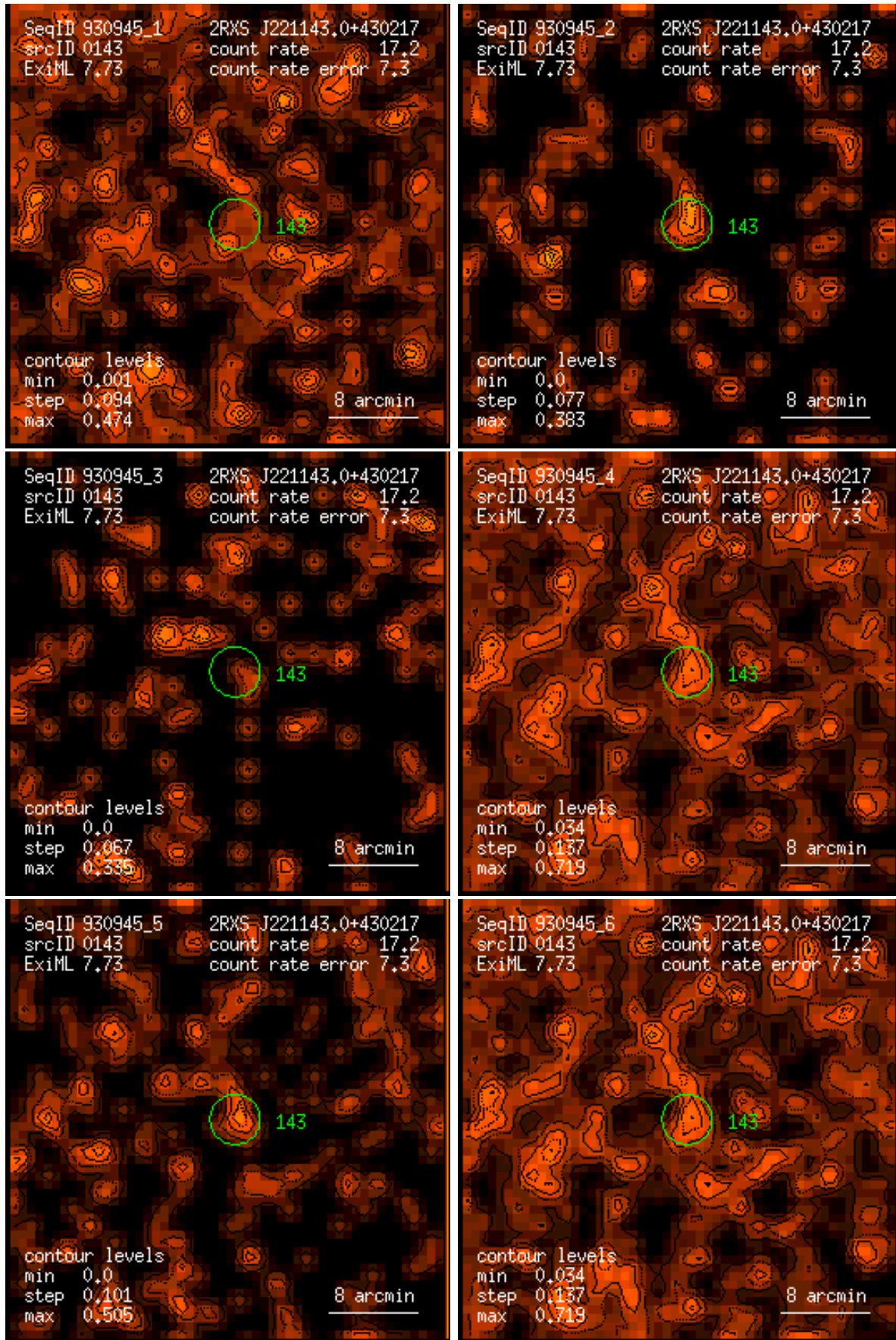
Figure 143: RASS 930945: detection 0143: band rate images, Gaussian filter: (1) PSPC channels 11 – 41, (2) 52 – 90, (3) 91 – 201, (4) 11 – 235, (5) 52 – 201, (6) 11 – 201. Broad band rates in counts/ks. Band rate contour levels in counts/ks/arcmin 2 .
