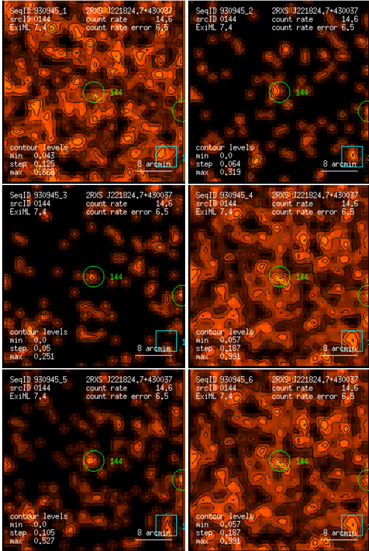
Figure 144: RASS 930945: detection 0144: band rate images, Gaussian filter: (1) PSPC channels 11 – 41, (2) 52 – 90, (3) 91 – 201, (4) 11 – 235, (5) 52 – 201, (6) 11 – 201. Broad band rates in counts/ks. Band rate contour levels in counts/ks/arcmin 2 .
