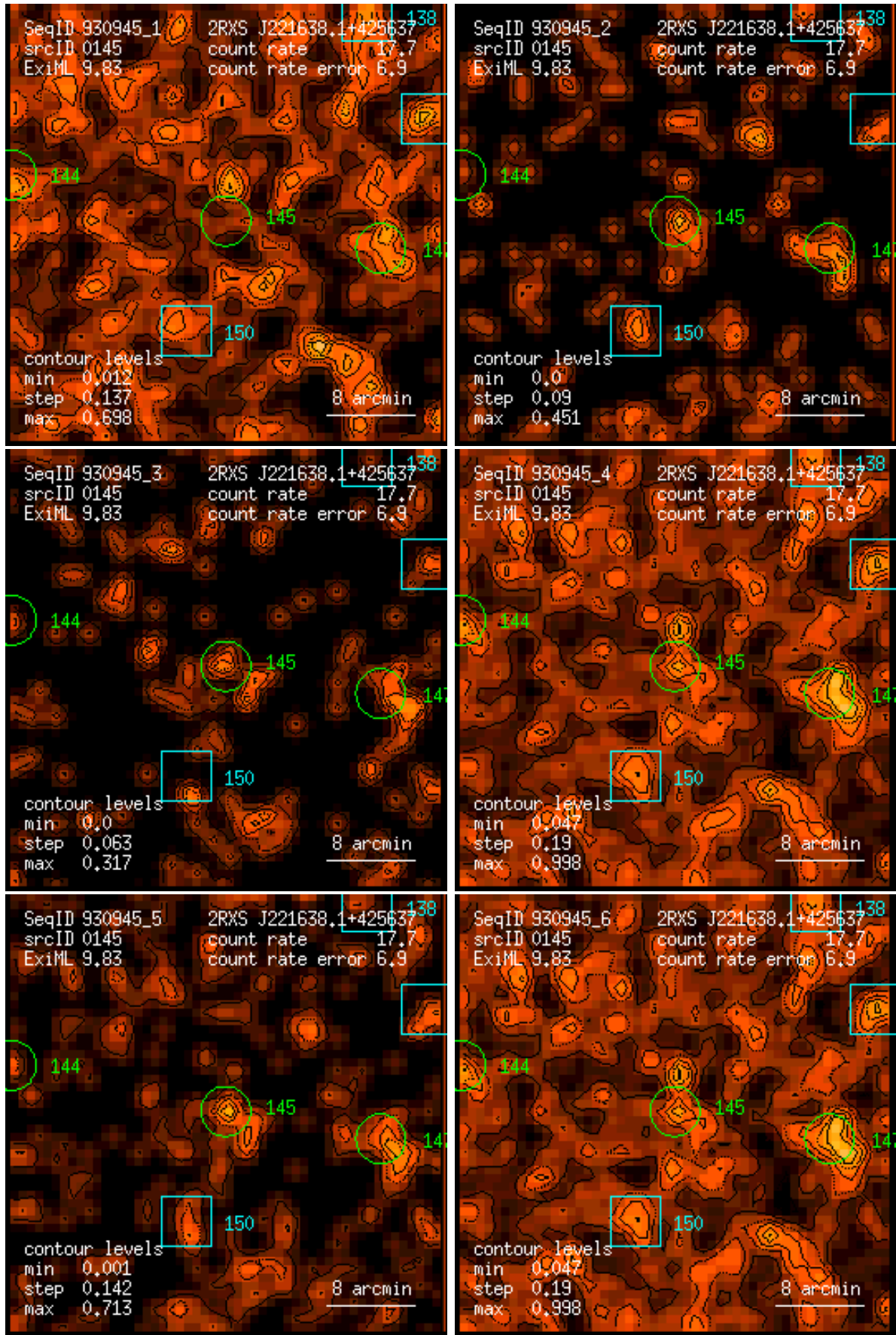
Figure 145: RASS 930945: detection 0145: band rate images, Gaussian filter: (1) PSPC channels 11 – 41, (2) 52 – 90, (3) 91 – 201, (4) 11 – 235, (5) 52 – 201, (6) 11 – 201. Broad band rates in counts/ks. Band rate contour levels in counts/ks/arcmin 2 .
