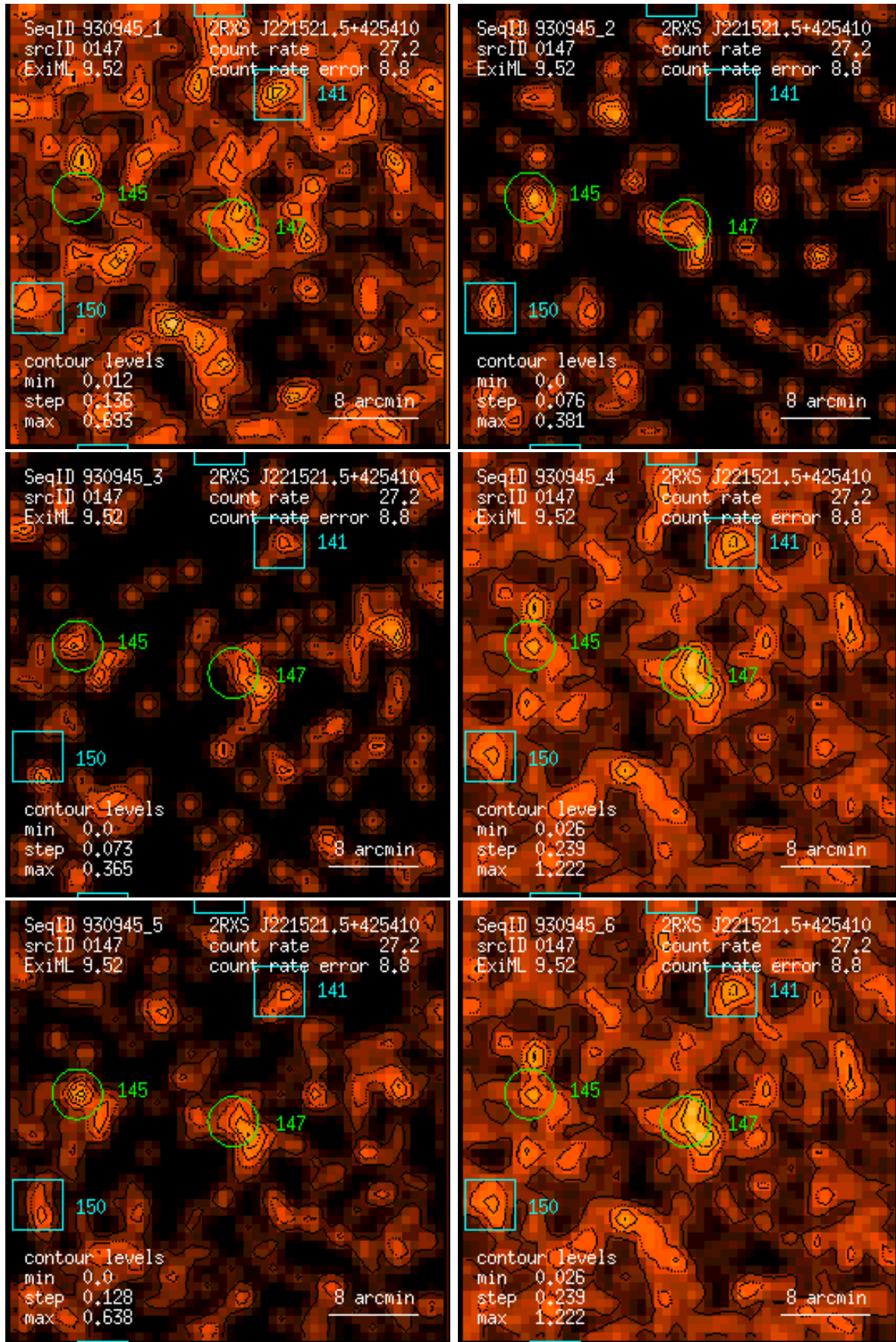
Figure 147: RASS 930945: detection 0147: band rate images, Gaussian filter: (1) PSPC channels 11 – 41, (2) 52 – 90, (3) 91 – 201, (4) 11 – 235, (5) 52 – 201, (6) 11 – 201. Broad band rates in counts/ks. Band rate contour levels in counts/ks/arcmin 2 .
