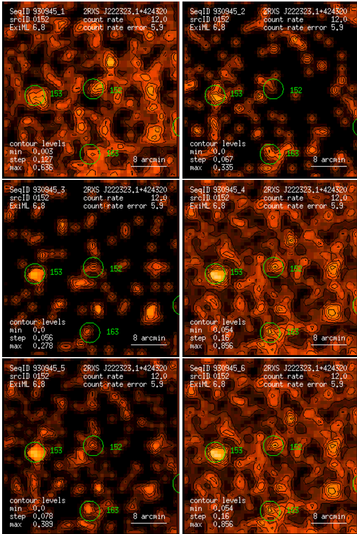
Figure 152: RASS 930945: detection 0152: band rate images, Gaussian filter: (1) PSPC channels 11 – 41, (2) 52 – 90, (3) 91 – 201, (4) 11 – 235, (5) 52 – 201, (6) 11 – 201. Broad band rates in counts/ks. Band rate contour levels in counts/ks/arcmin 2 .
