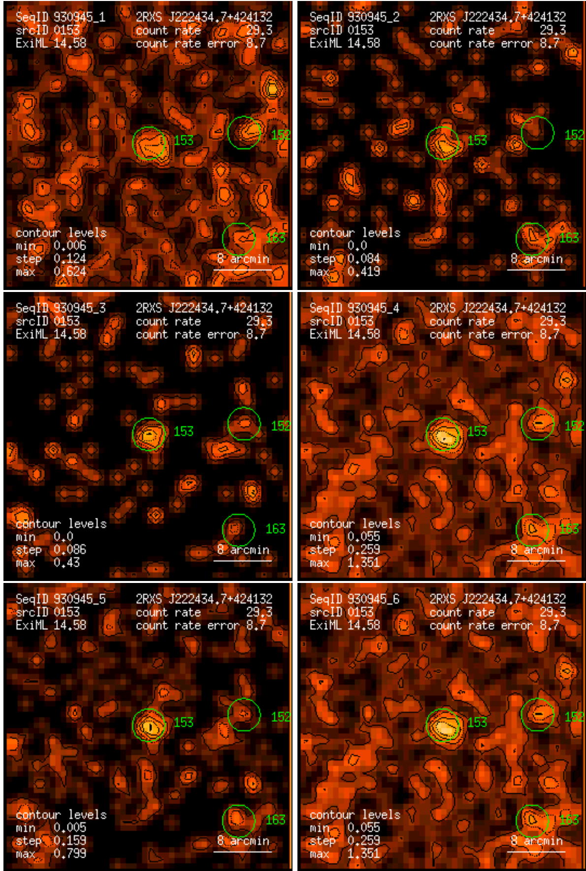
Figure 153: RASS 930945: detection 0153: band rate images, Gaussian filter: (1) PSPC channels 11 – 41, (2) 52 – 90, (3) 91 – 201, (4) 11 – 235, (5) 52 – 201, (6) 11 – 201. Broad band rates in counts/ks. Band rate contour levels in counts/ks/arcmin 2 .
