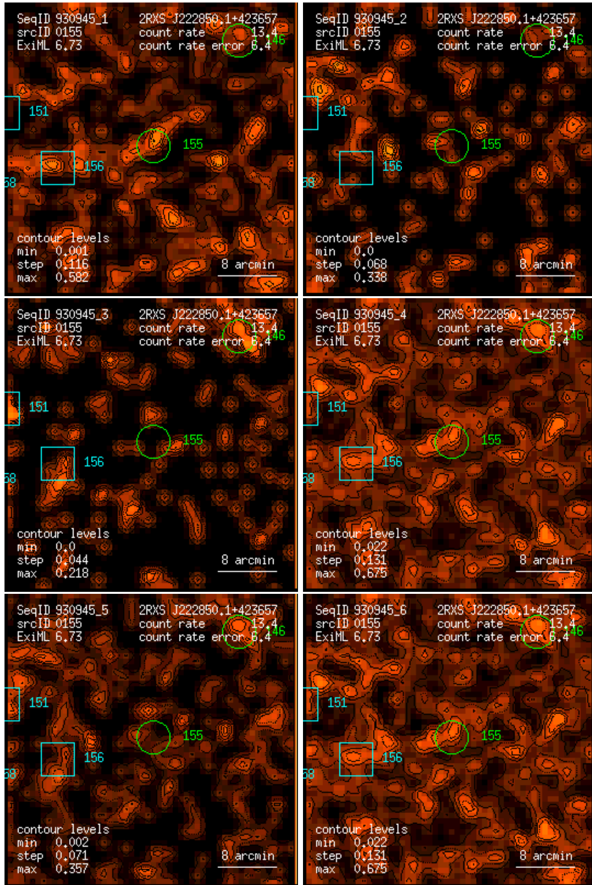
Figure 155: RASS 930945: detection 0155: band rate images, Gaussian filter: (1) PSPC channels 11 – 41, (2) 52 – 90, (3) 91 – 201, (4) 11 – 235, (5) 52 – 201, (6) 11 – 201. Broad band rates in counts/ks. Band rate contour levels in counts/ks/arcmin 2 .
