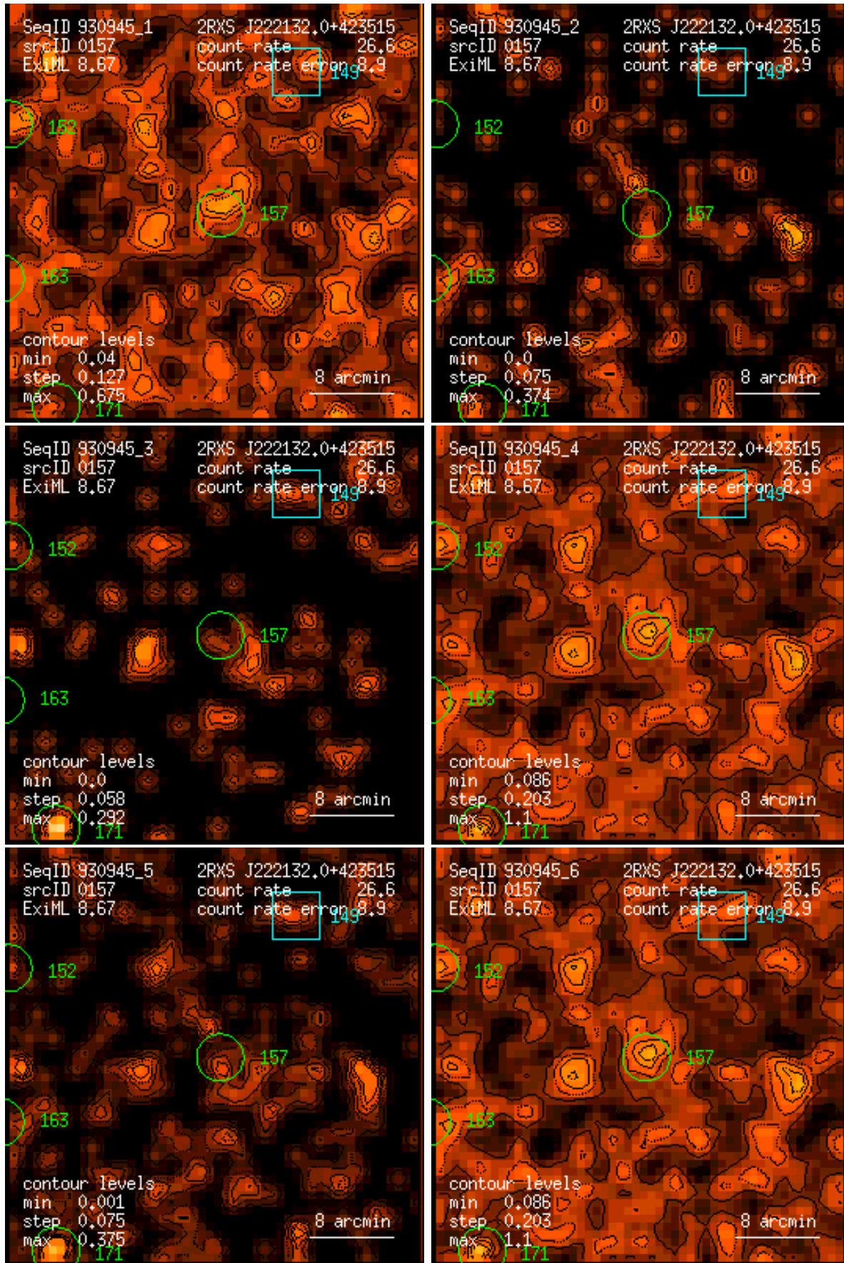
Figure 157: RASS 930945: detection 0157: band rate images, Gaussian filter: (1) PSPC channels 11 – 41, (2) 52 – 90, (3) 91 – 201, (4) 11 – 235, (5) 52 – 201, (6) 11 – 201. Broad band rates in counts/ks. Band rate contour levels in counts/ks/arcmin 2 .
