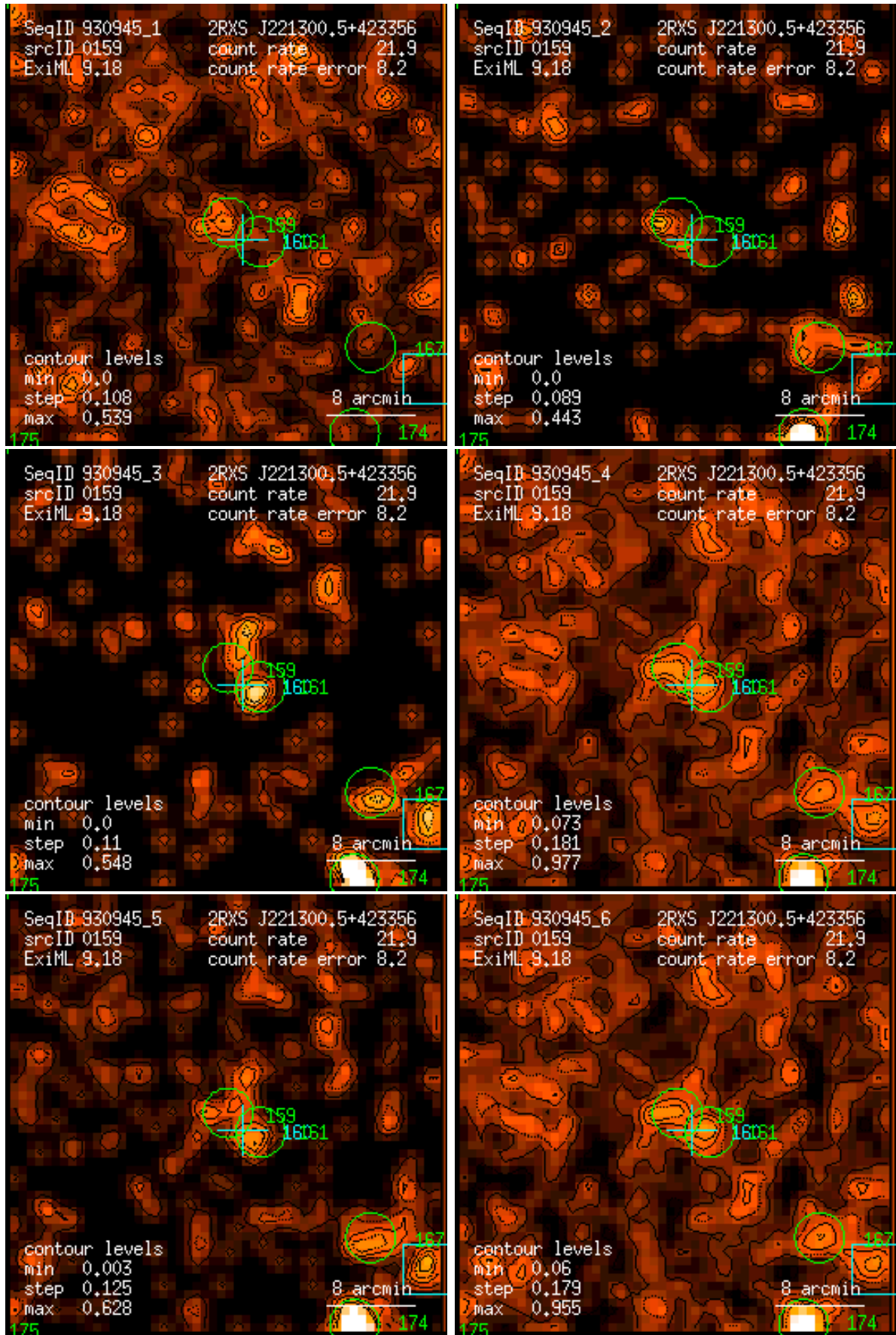
Figure 159: RASS 930945: detection 0159: band rate images, Gaussian filter: (1) PSPC channels 11 – 41, (2) 52 – 90, (3) 91 – 201, (4) 11 – 235, (5) 52 – 201, (6) 11 – 201. Broad band rates in counts/ks. Band rate contour levels in counts/ks/arcmin 2 .
