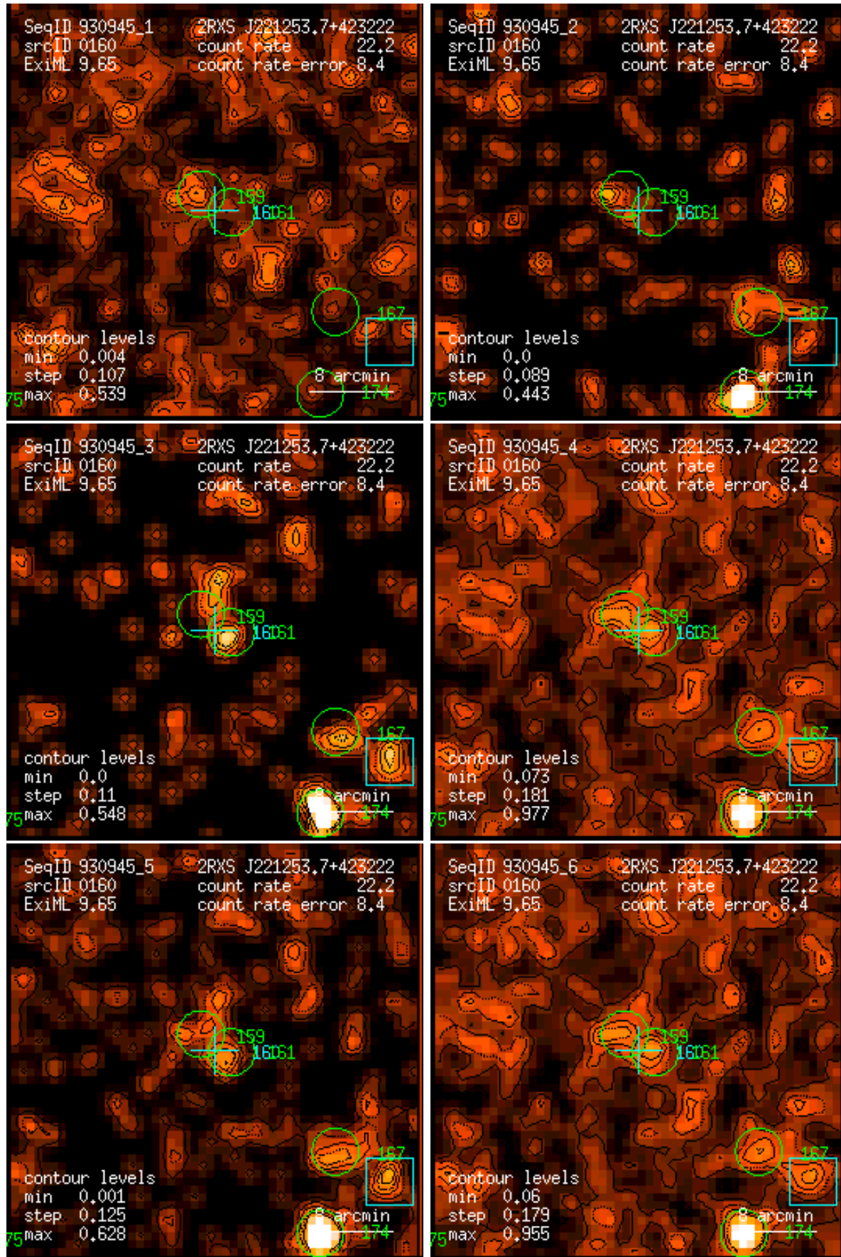
Figure 160: RASS 930945: detection 0160: band rate images, Gaussian filter: (1) PSPC channels 11 – 41, (2) 52 – 90, (3) 91 – 201, (4) 11 – 235, (5) 52 – 201, (6) 11 – 201. Broad band rates in counts/ks. Band rate contour levels in counts/ks/arcmin 2 .
