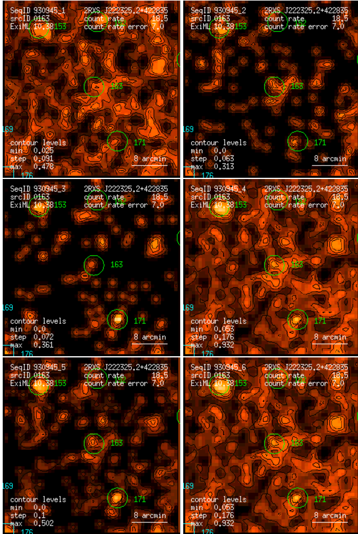
Figure 163: RASS 930945: detection 0163: band rate images, Gaussian filter: (1) PSPC channels 11 – 41, (2) 52 – 90, (3) 91 – 201, (4) 11 – 235, (5) 52 – 201, (6) 11 – 201. Broad band rates in counts/ks. Band rate contour levels in counts/ks/arcmin 2 .
