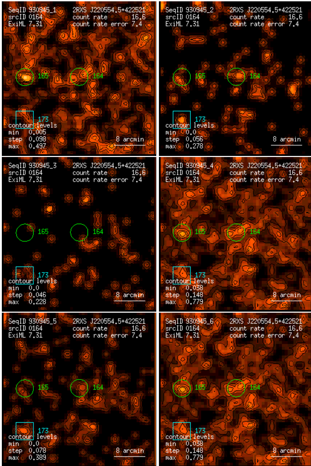
Figure 164: RASS 930945: detection 0164: band rate images, Gaussian filter: (1) PSPC channels 11 – 41, (2) 52 – 90, (3) 91 – 201, (4) 11 – 235, (5) 52 – 201, (6) 11 – 201. Broad band rates in counts/ks. Band rate contour levels in counts/ks/arcmin 2 .
