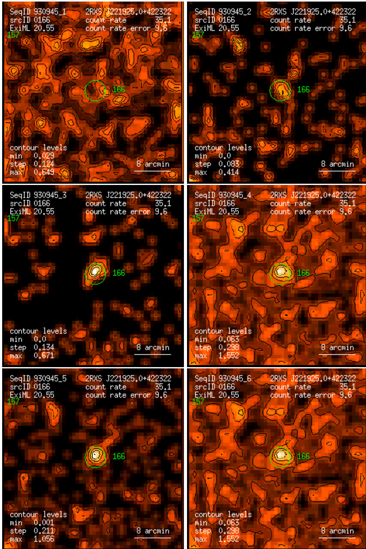
Figure 166: RASS 930945: detection 0166: band rate images, Gaussian filter: (1) PSPC channels 11 – 41, (2) 52 – 90, (3) 91 – 201, (4) 11 – 235, (5) 52 – 201, (6) 11 – 201. Broad band rates in counts/ks. Band rate contour levels in counts/ks/arcmin 2 .
