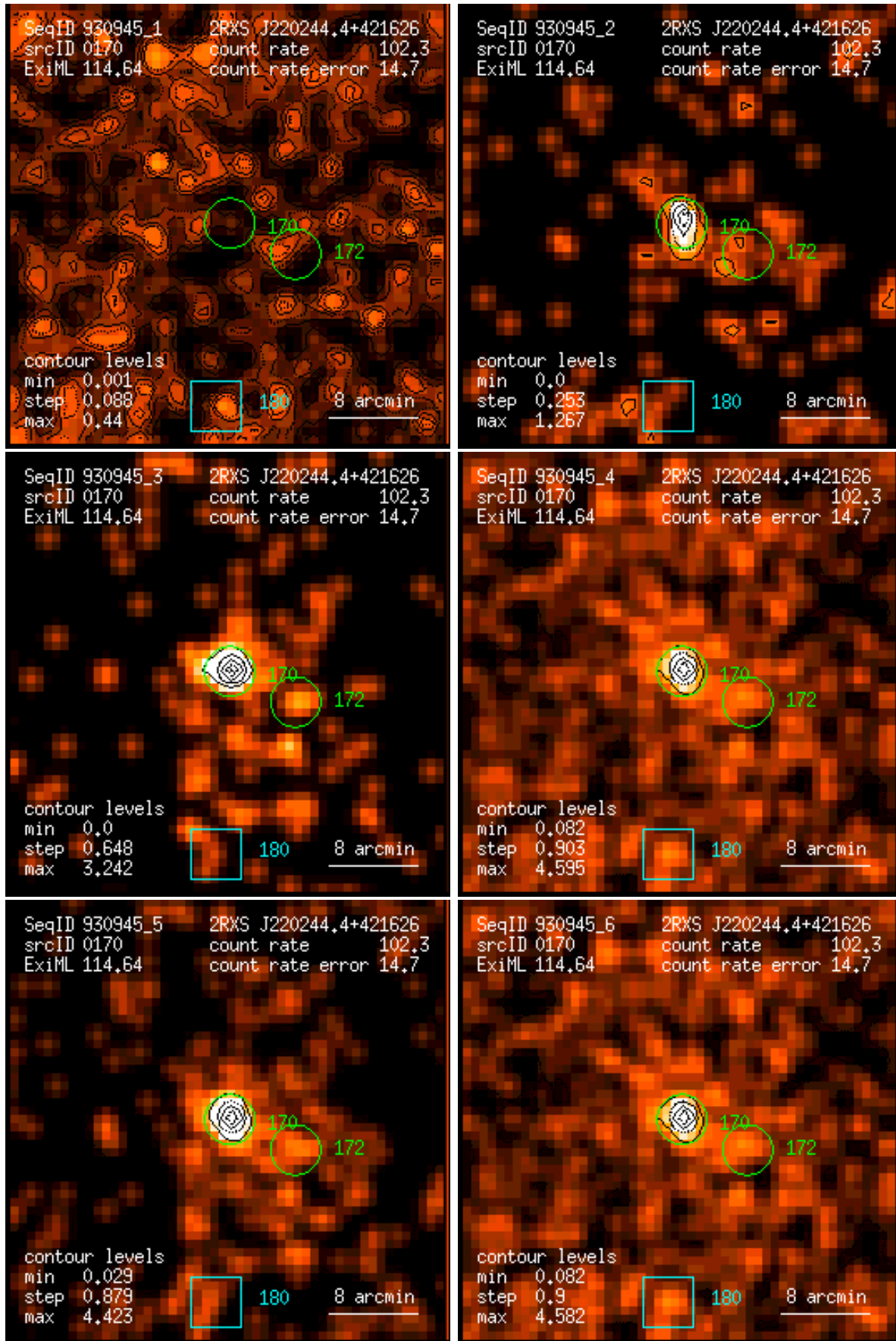
Figure 170: RASS 930945: detection 0170: band rate images, Gaussian filter: (1) PSPC channels 11 – 41, (2) 52 – 90, (3) 91 – 201, (4) 11 – 235, (5) 52 – 201, (6) 11 – 201. Broad band rates in counts/ks. Band rate contour levels in counts/ks/arcmin 2 .
