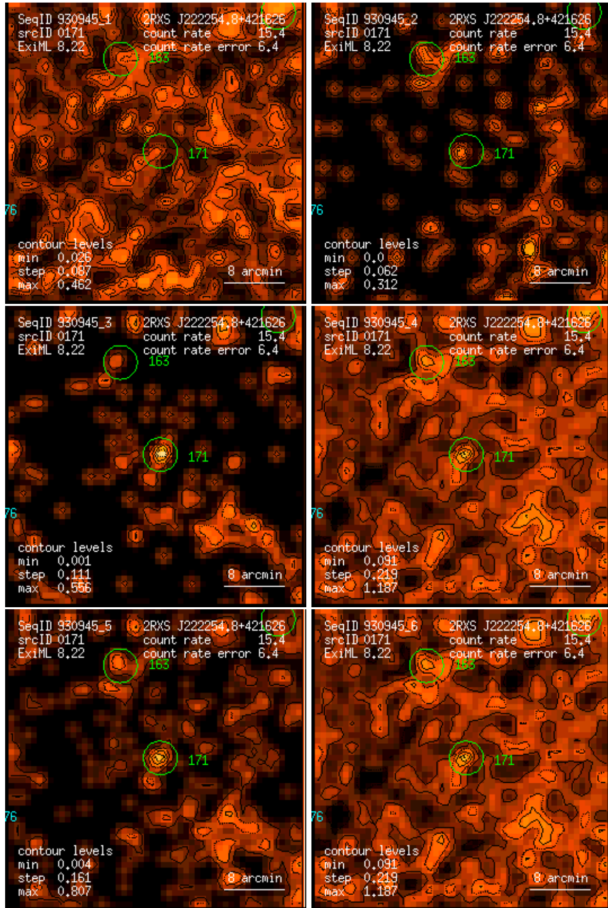
Figure 171: RASS 930945: detection 0171: band rate images, Gaussian filter: (1) PSPC channels 11 – 41, (2) 52 – 90, (3) 91 – 201, (4) 11 – 235, (5) 52 – 201, (6) 11 – 201. Broad band rates in counts/ks. Band rate contour levels in counts/ks/arcmin 2 .
