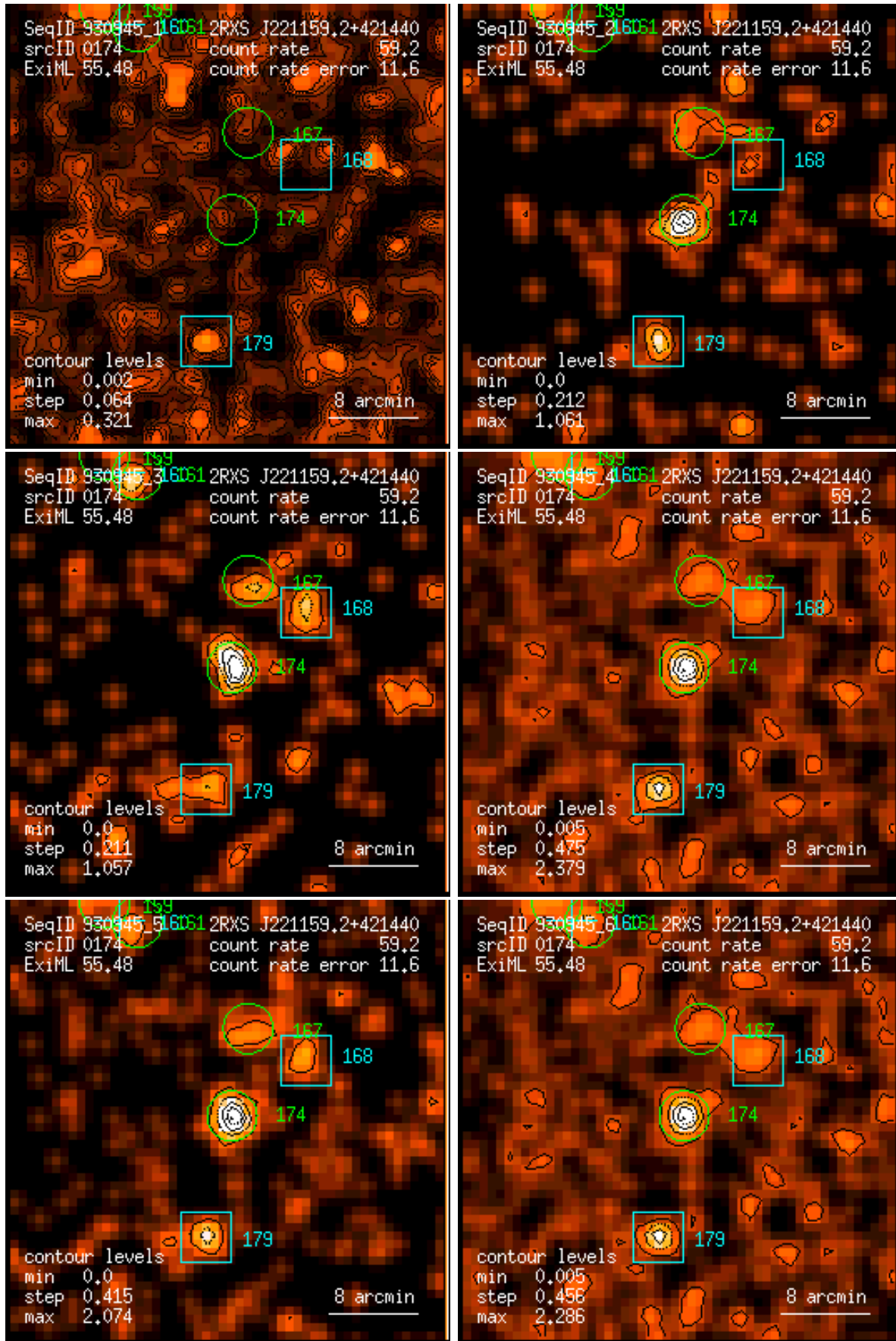
Figure 174: RASS 930945: detection 0174: band rate images, Gaussian filter: (1) PSPC channels 11 – 41, (2) 52 – 90, (3) 91 – 201, (4) 11 – 235, (5) 52 – 201, (6) 11 – 201. Broad band rates in counts/ks. Band rate contour levels in counts/ks/arcmin 2 .
