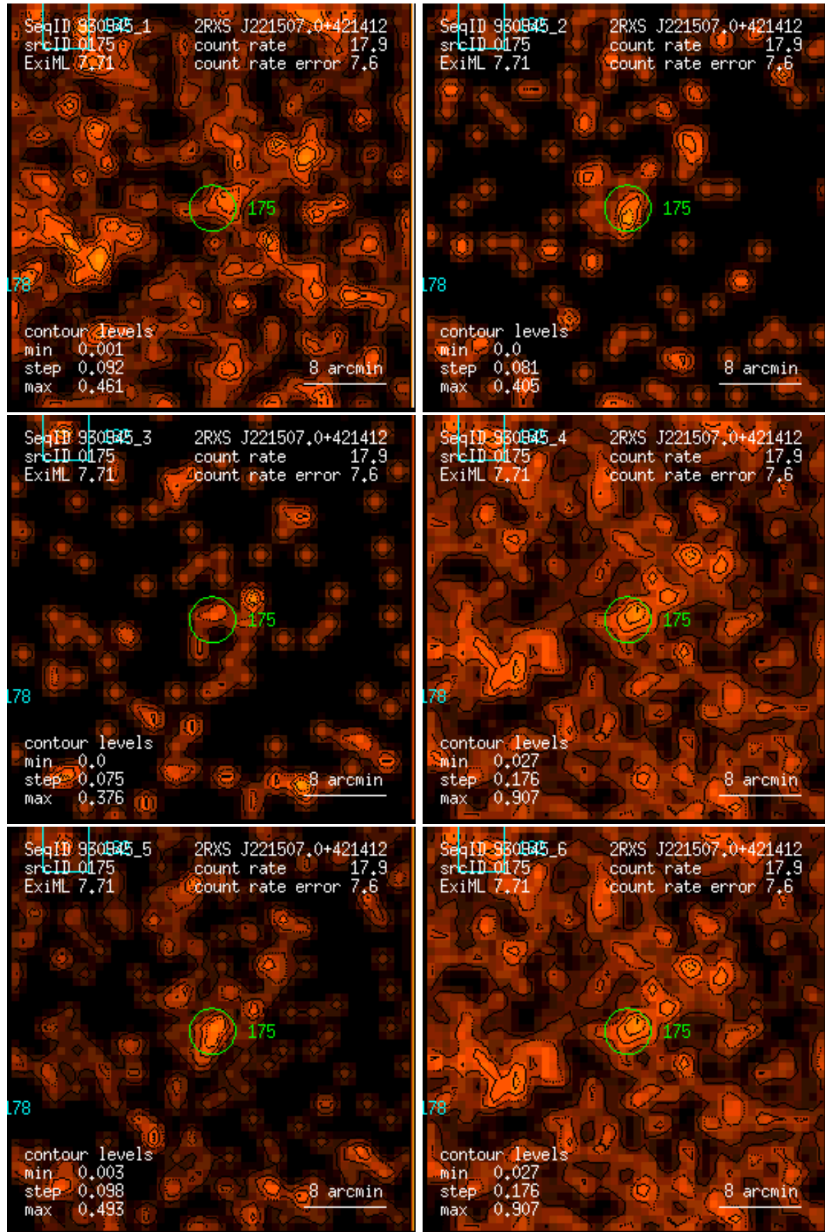
Figure 175: RASS 930945: detection 0175: band rate images, Gaussian filter: (1) PSPC channels 11 – 41, (2) 52 – 90, (3) 91 – 201, (4) 11 – 235, (5) 52 – 201, (6) 11 – 201. Broad band rates in counts/ks. Band rate contour levels in counts/ks/arcmin 2 .
