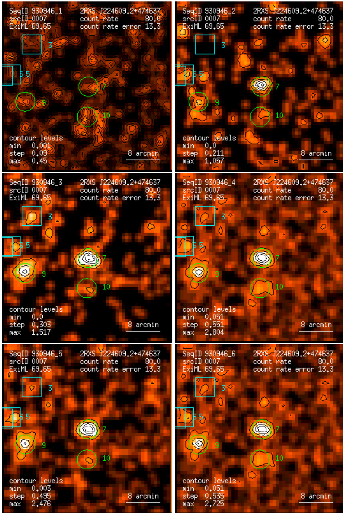
Figure 7: RASS 930946: detection 0007: band rate images, Gaussian filter: (1) PSPC channels 11 – 41, (2) 52 – 90, (3) 91 – 201, (4) 11 – 235, (5) 52 – 201, (6) 11 – 201. Broad band rates in counts/ks. Band rate contour levels in counts/ks/arcmin 2 .
