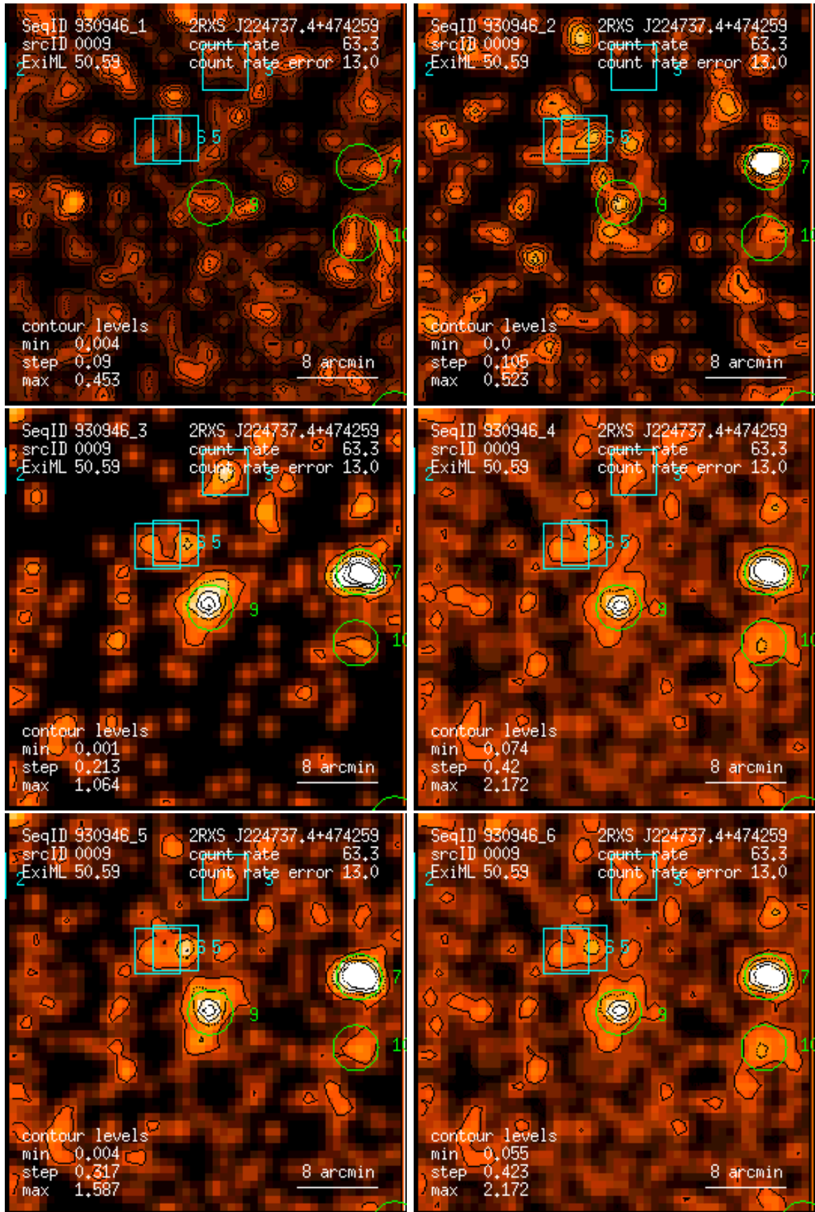
Figure 9: RASS 930946: detection 0009: band rate images, Gaussian filter: (1) PSPC channels 11 – 41, (2) 52 – 90, (3) 91 – 201, (4) 11 – 235, (5) 52 – 201, (6) 11 – 201. Broad band rates in counts/ks. Band rate contour levels in counts/ks/arcmin 2 .
