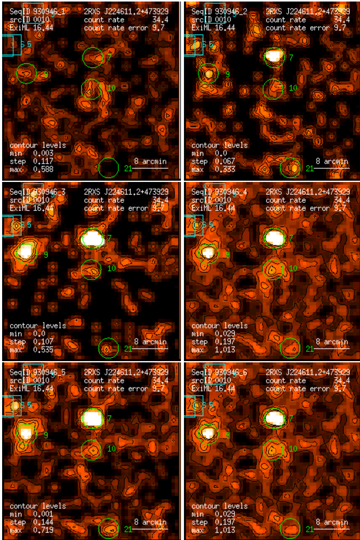
Figure 10: RASS 930946: detection 0010: band rate images, Gaussian filter: (1) PSPC channels 11 – 41, (2) 52 – 90, (3) 91 – 201, (4) 11 – 235, (5) 52 – 201, (6) 11 – 201. Broad band rates in counts/ks. Band rate contour levels in counts/ks/arcmin 2 .
