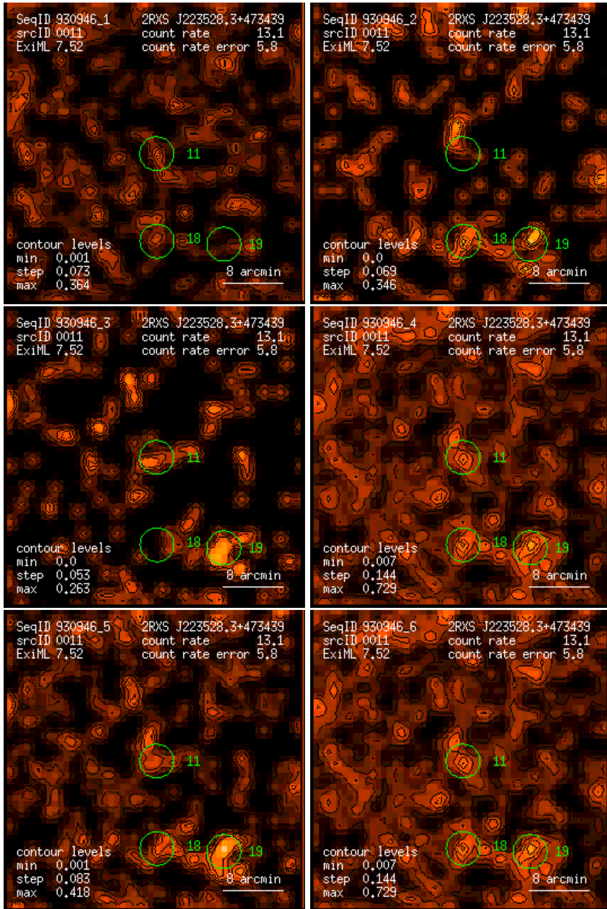
Figure 11: RASS 930946: detection 0011: band rate images, Gaussian filter: (1) PSPC channels 11 – 41, (2) 52 – 90, (3) 91 – 201, (4) 11 – 235, (5) 52 – 201, (6) 11 – 201. Broad band rates in counts/ks. Band rate contour levels in counts/ks/arcmin 2 .
