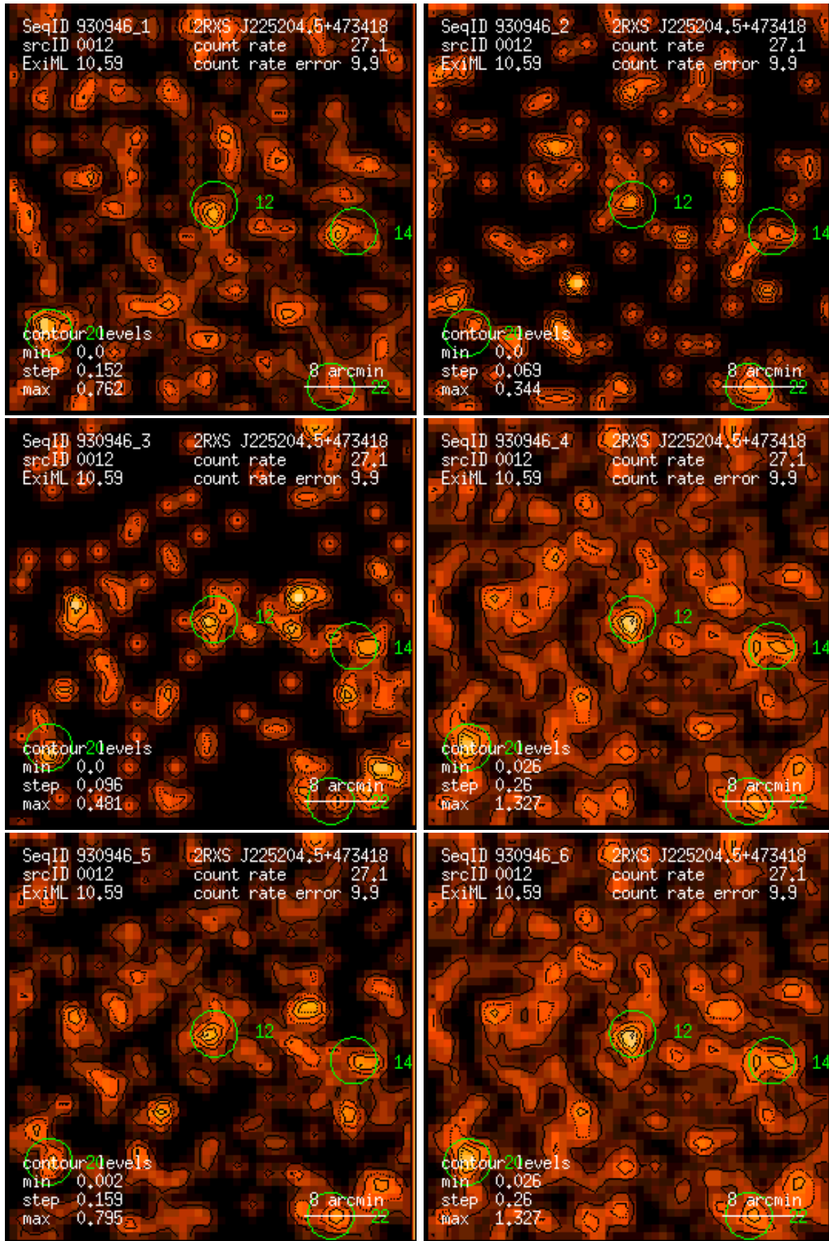
Figure 12: RASS 930946: detection 0012: band rate images, Gaussian filter: (1) PSPC channels 11 – 41, (2) 52 – 90, (3) 91 – 201, (4) 11 – 235, (5) 52 – 201, (6) 11 – 201. Broad band rates in counts/ks. Band rate contour levels in counts/ks/arcmin 2 .
