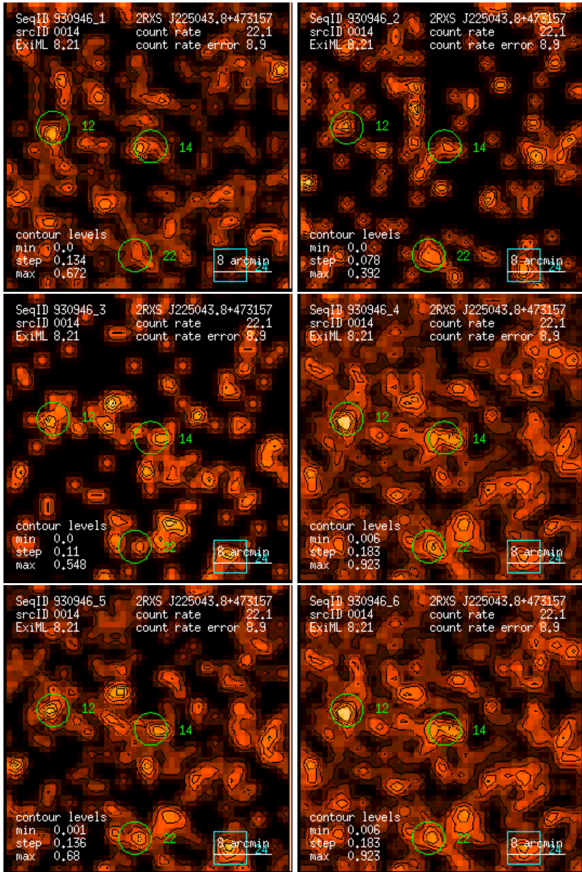
Figure 14: RASS 930946: detection 0014: band rate images, Gaussian filter: (1) PSPC channels 11 – 41, (2) 52 – 90, (3) 91 – 201, (4) 11 – 235, (5) 52 – 201, (6) 11 – 201. Broad band rates in counts/ks. Band rate contour levels in counts/ks/arcmin 2 .
