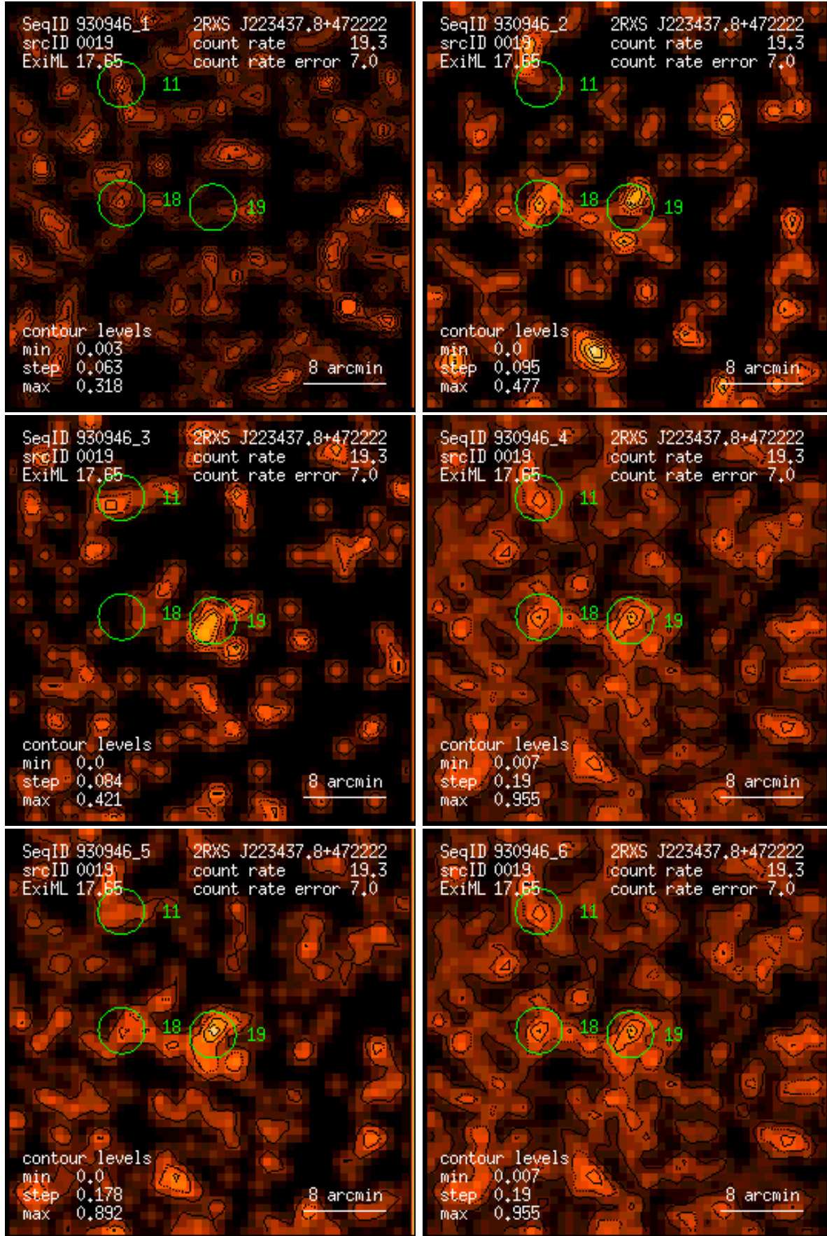
Figure 19: RASS 930946: detection 0019: band rate images, Gaussian filter: (1) PSPC channels 11 – 41, (2) 52 – 90, (3) 91 – 201, (4) 11 – 235, (5) 52 – 201, (6) 11 – 201. Broad band rates in counts/ks. Band rate contour levels in counts/ks/arcmin 2 .
