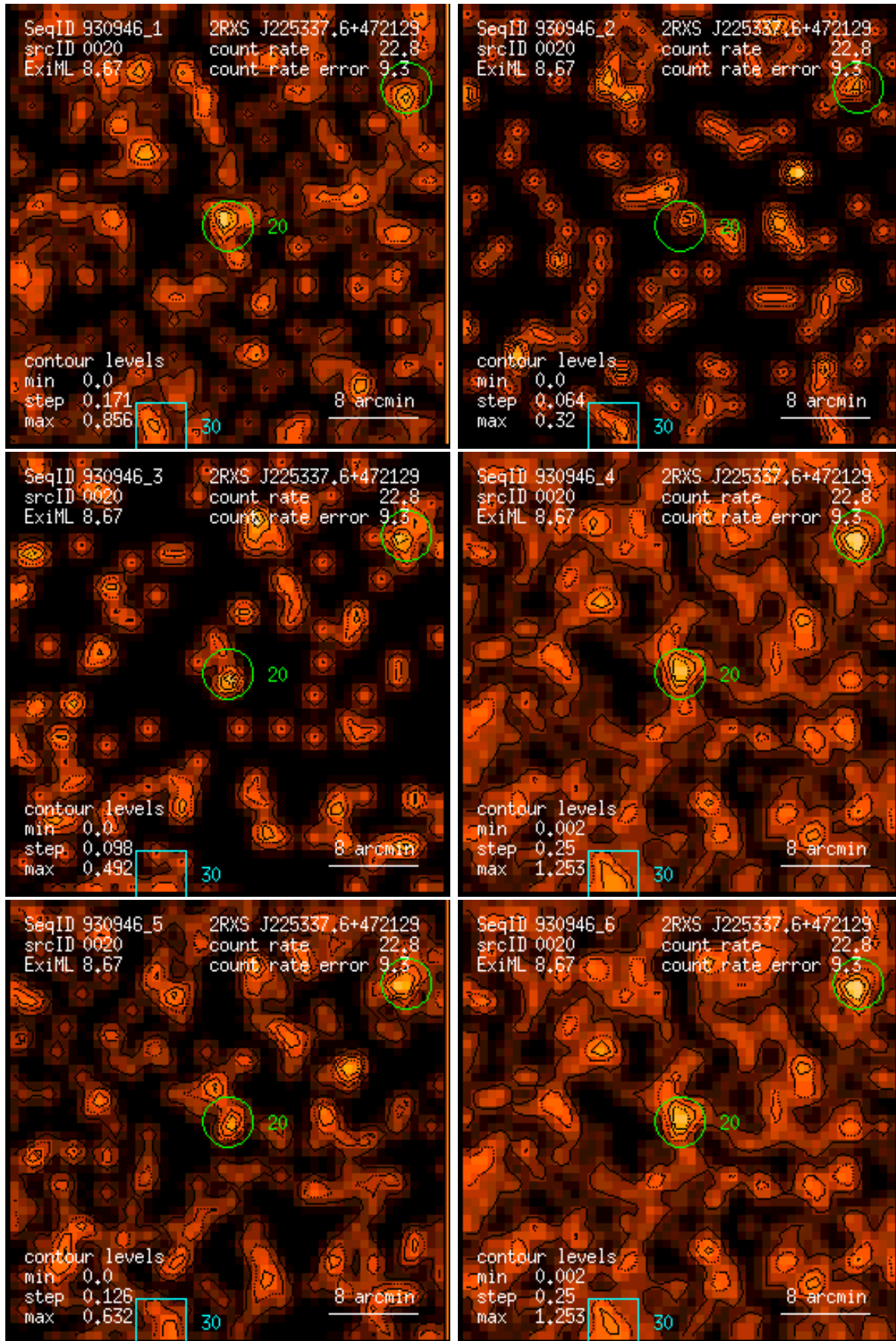
Figure 20: RASS 930946: detection 0020: band rate images, Gaussian filter: (1) PSPC channels 11 – 41, (2) 52 – 90, (3) 91 – 201, (4) 11 – 235, (5) 52 – 201, (6) 11 – 201. Broad band rates in counts/ks. Band rate contour levels in counts/ks/arcmin 2 .
