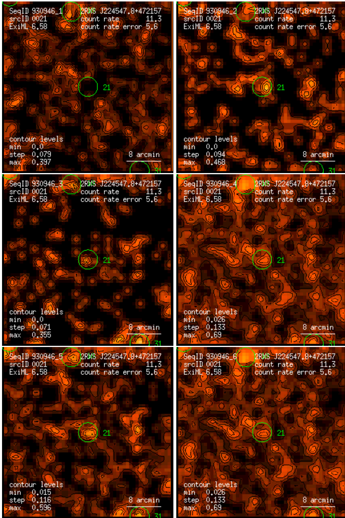
Figure 21: RASS 930946: detection 0021: band rate images, Gaussian filter: (1) PSPC channels 11 – 41, (2) 52 – 90, (3) 91 – 201, (4) 11 – 235, (5) 52 – 201, (6) 11 – 201. Broad band rates in counts/ks. Band rate contour levels in counts/ks/arcmin 2 .
