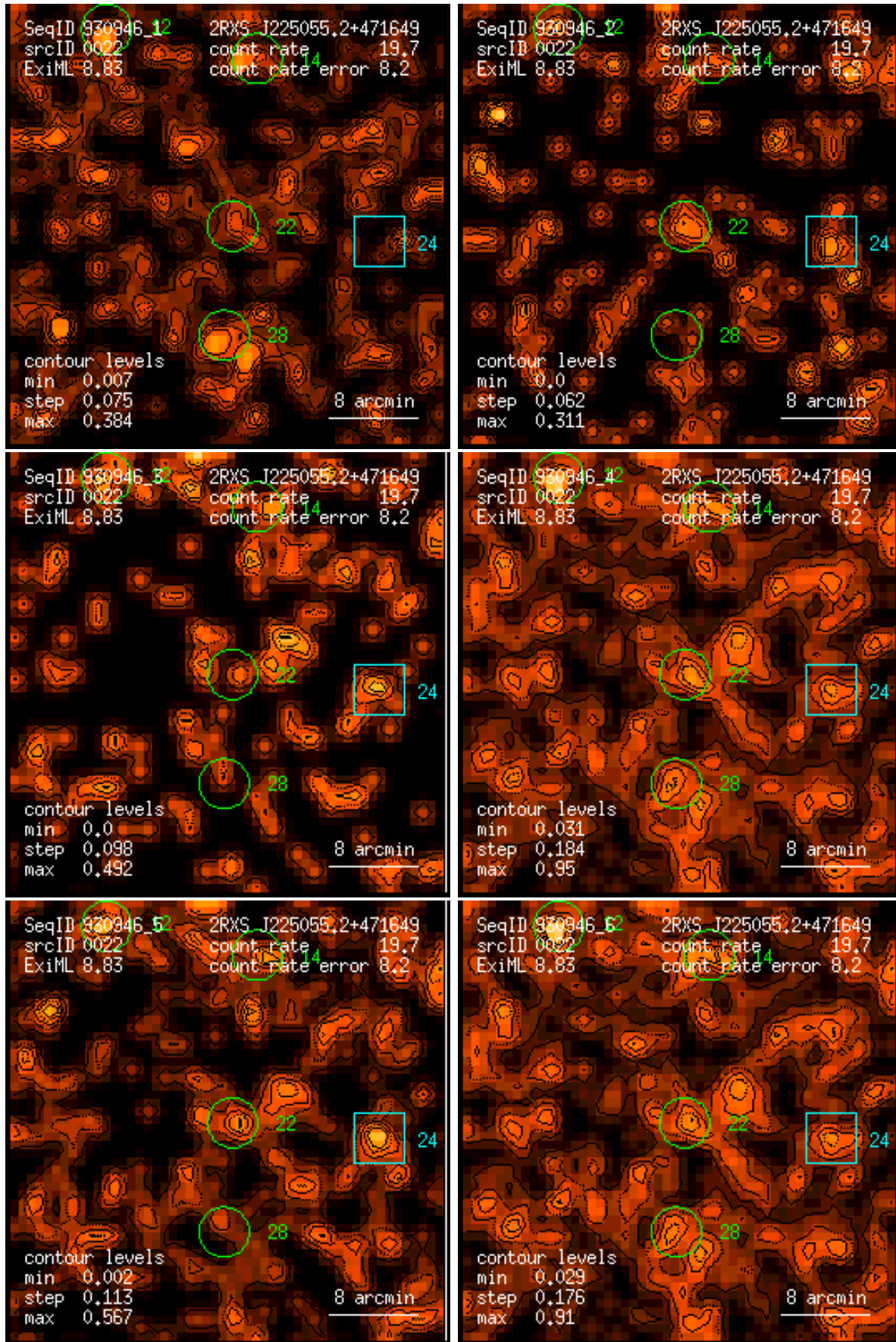
Figure 22: RASS 930946: detection 0022: band rate images, Gaussian filter: (1) PSPC channels 11 – 41, (2) 52 – 90, (3) 91 – 201, (4) 11 – 235, (5) 52 – 201, (6) 11 – 201. Broad band rates in counts/ks. Band rate contour levels in counts/ks/arcmin 2 .
