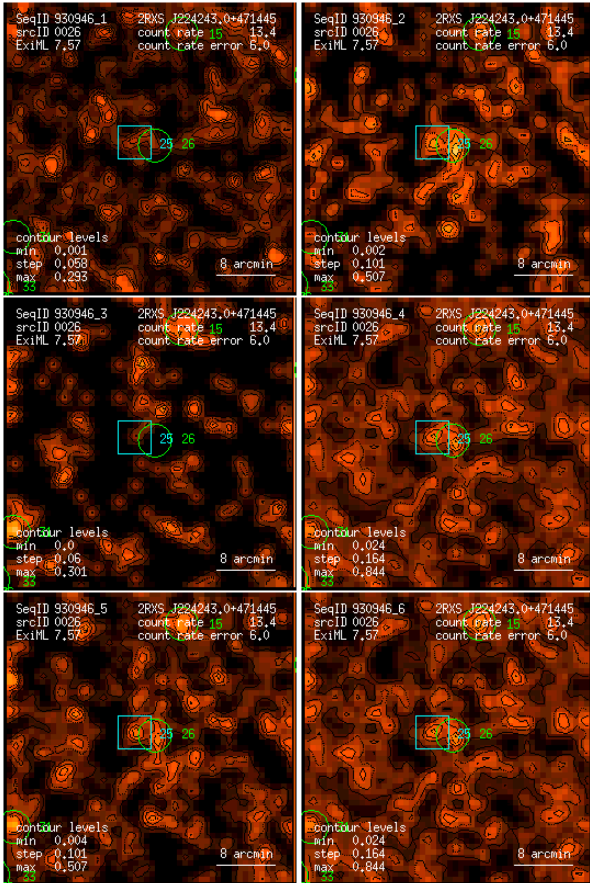
Figure 26: RASS 930946: detection 0026: band rate images, Gaussian filter: (1) PSPC channels 11 – 41, (2) 52 – 90, (3) 91 – 201, (4) 11 – 235, (5) 52 – 201, (6) 11 – 201. Broad band rates in counts/ks. Band rate contour levels in counts/ks/arcmin 2 .
