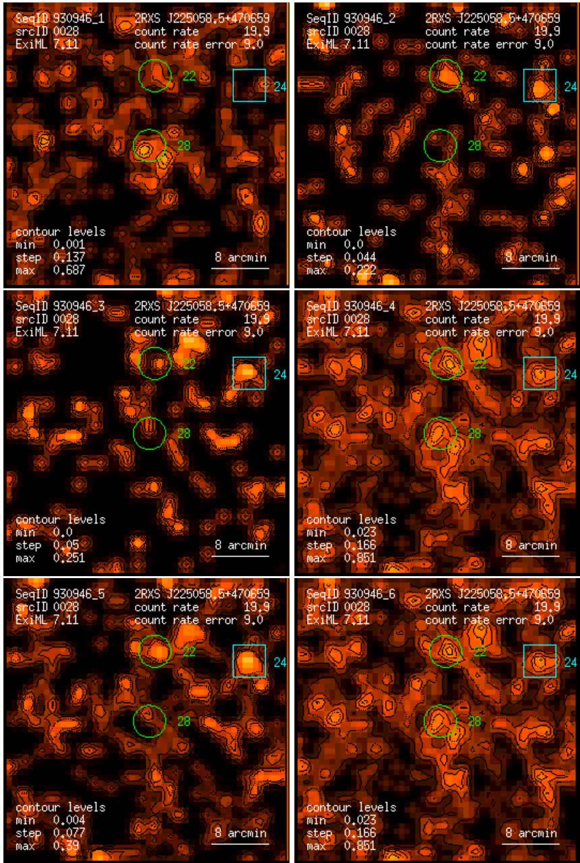
Figure 28: RASS 930946: detection 0028: band rate images, Gaussian filter: (1) PSPC channels 11 – 41, (2) 52 – 90, (3) 91 – 201, (4) 11 – 235, (5) 52 – 201, (6) 11 – 201. Broad band rates in counts/ks. Band rate contour levels in counts/ks/arcmin 2 .
