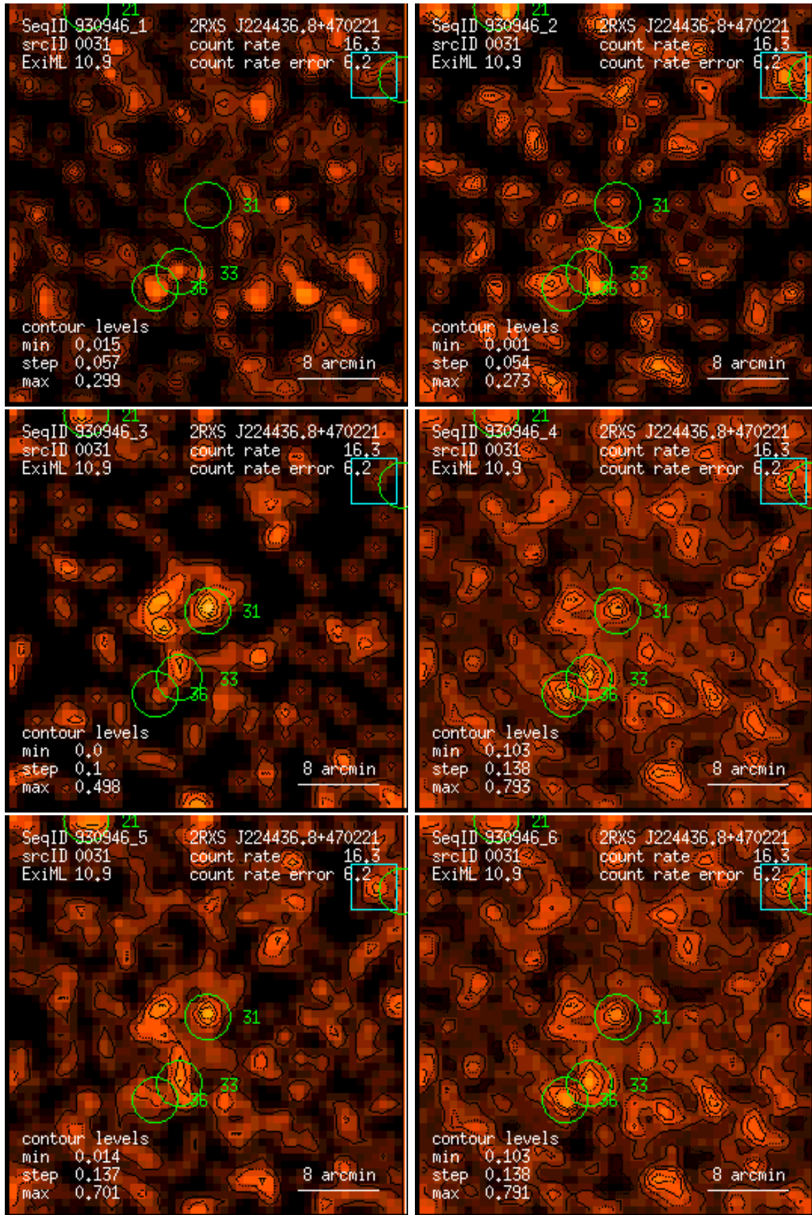
Figure 31: RASS 930946: detection 0031: band rate images, Gaussian filter: (1) PSPC channels 11 – 41, (2) 52 – 90, (3) 91 – 201, (4) 11 – 235, (5) 52 – 201, (6) 11 – 201. Broad band rates in counts/ks. Band rate contour levels in counts/ks/arcmin 2 .
