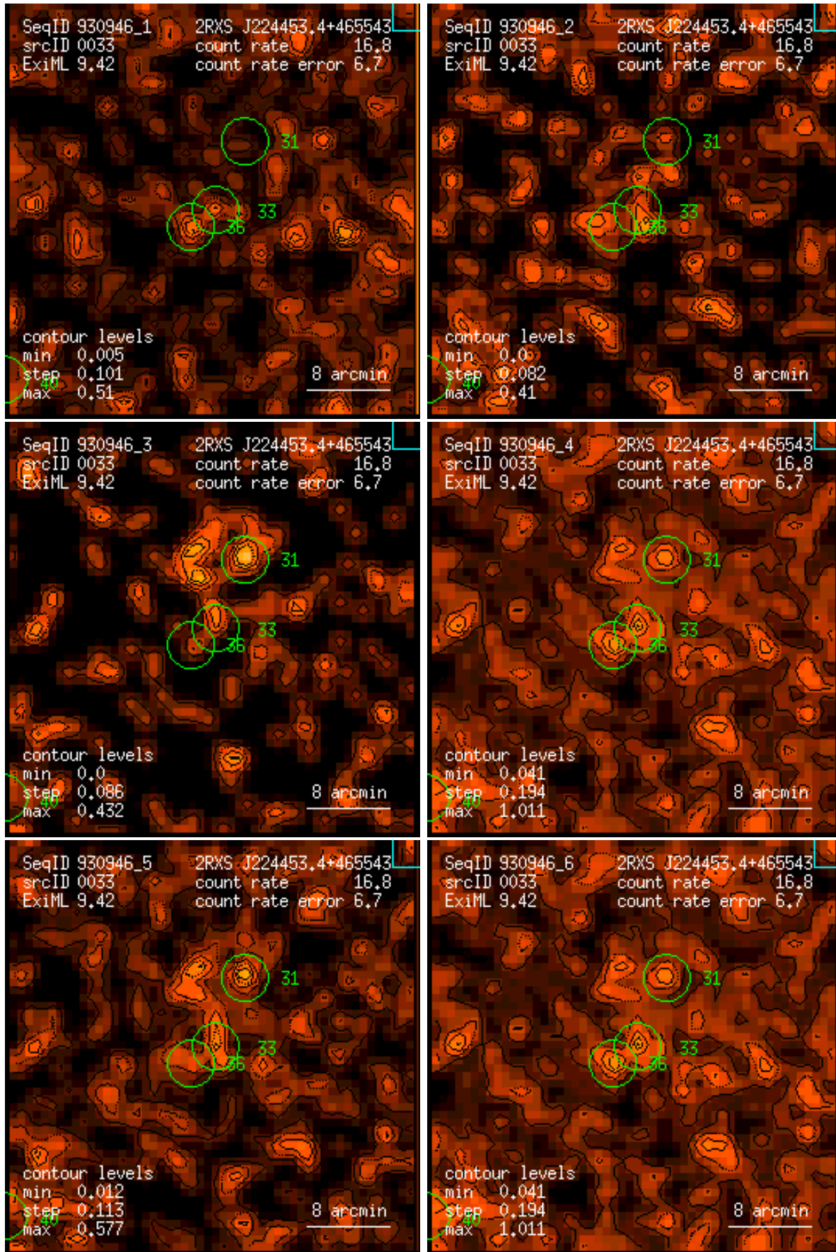
Figure 33: RASS 930946: detection 0033: band rate images, Gaussian filter: (1) PSPC channels 11 – 41, (2) 52 – 90, (3) 91 – 201, (4) 11 – 235, (5) 52 – 201, (6) 11 – 201. Broad band rates in counts/ks. Band rate contour levels in counts/ks/arcmin 2 .
