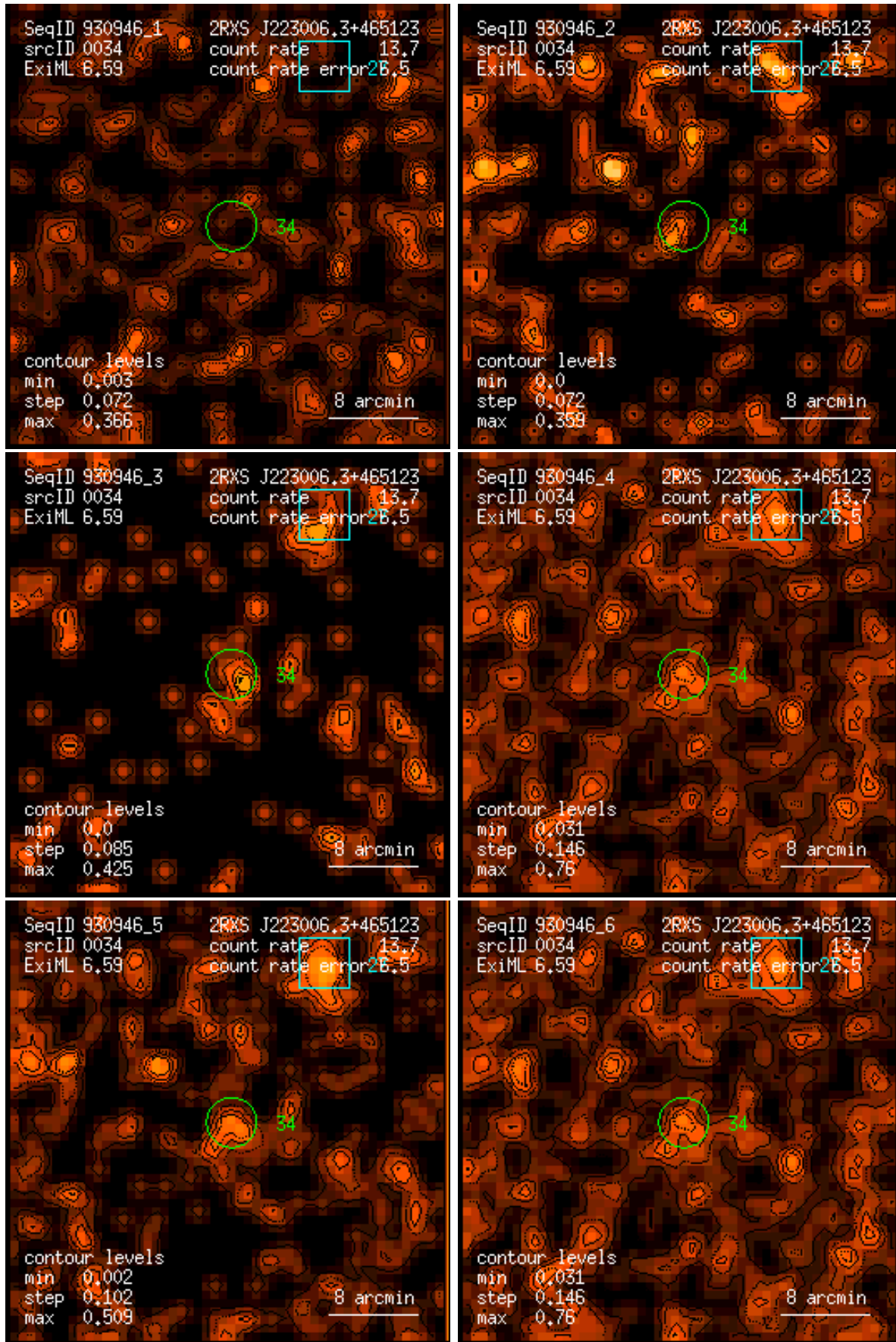
Figure 34: RASS 930946: detection 0034: band rate images, Gaussian filter: (1) PSPC channels 11 – 41, (2) 52 – 90, (3) 91 – 201, (4) 11 – 235, (5) 52 – 201, (6) 11 – 201. Broad band rates in counts/ks. Band rate contour levels in counts/ks/arcmin 2 .
