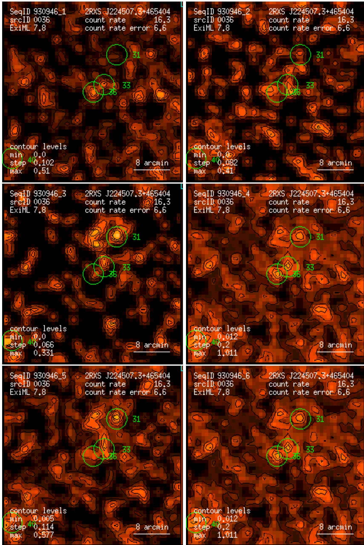
Figure 36: RASS 930946: detection 0036: band rate images, Gaussian filter: (1) PSPC channels 11 – 41, (2) 52 – 90, (3) 91 – 201, (4) 11 – 235, (5) 52 – 201, (6) 11 – 201. Broad band rates in counts/ks. Band rate contour levels in counts/ks/arcmin 2 .
