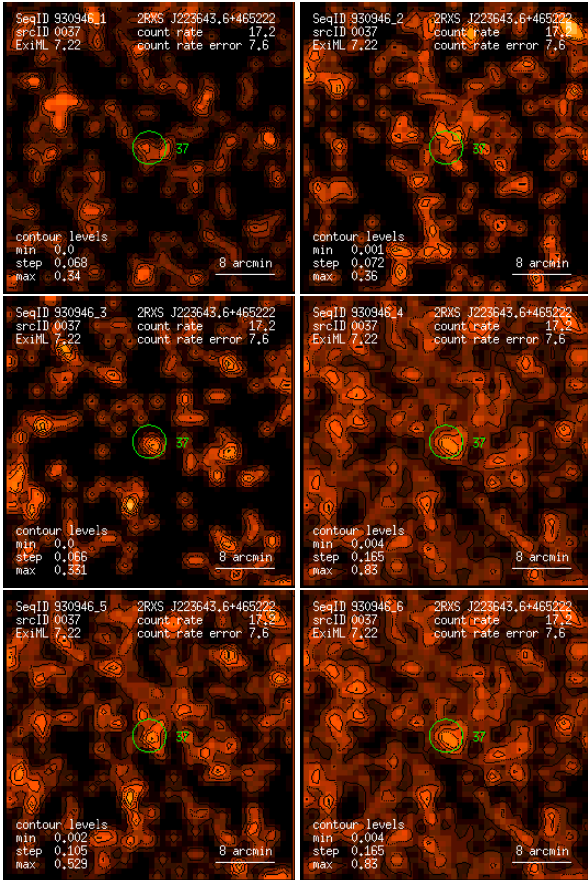
Figure 37: RASS 930946: detection 0037: band rate images, Gaussian filter: (1) PSPC channels 11 – 41, (2) 52 – 90, (3) 91 – 201, (4) 11 – 235, (5) 52 – 201, (6) 11 – 201. Broad band rates in counts/ks. Band rate contour levels in counts/ks/arcmin 2 .
