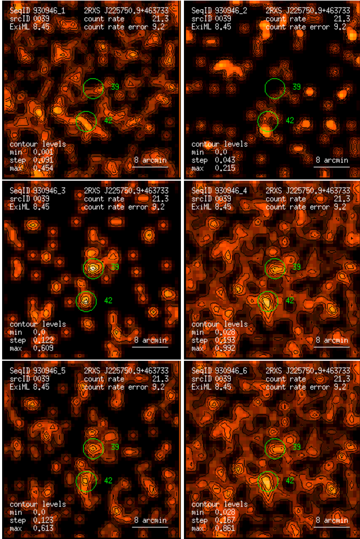
Figure 39: RASS 930946: detection 0039: band rate images, Gaussian filter: (1) PSPC channels 11 – 41, (2) 52 – 90, (3) 91 – 201, (4) 11 – 235, (5) 52 – 201, (6) 11 – 201. Broad band rates in counts/ks. Band rate contour levels in counts/ks/arcmin 2 .
