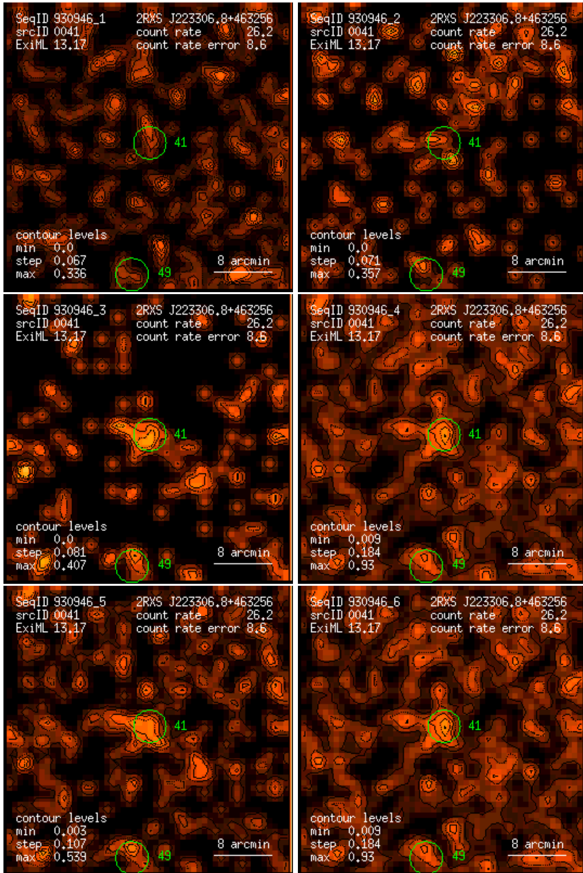
Figure 41: RASS 930946: detection 0041: band rate images, Gaussian filter: (1) PSPC channels 11 – 41, (2) 52 – 90, (3) 91 – 201, (4) 11 – 235, (5) 52 – 201, (6) 11 – 201. Broad band rates in counts/ks. Band rate contour levels in counts/ks/arcmin 2 .
