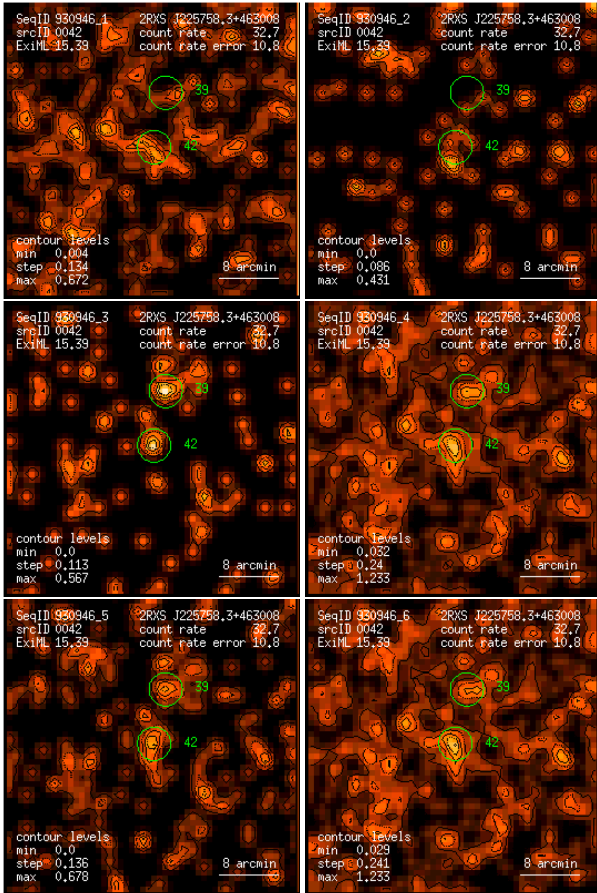
Figure 42: RASS 930946: detection 0042: band rate images, Gaussian filter: (1) PSPC channels 11 – 41, (2) 52 – 90, (3) 91 – 201, (4) 11 – 235, (5) 52 – 201, (6) 11 – 201. Broad band rates in counts/ks. Band rate contour levels in counts/ks/arcmin 2 .
