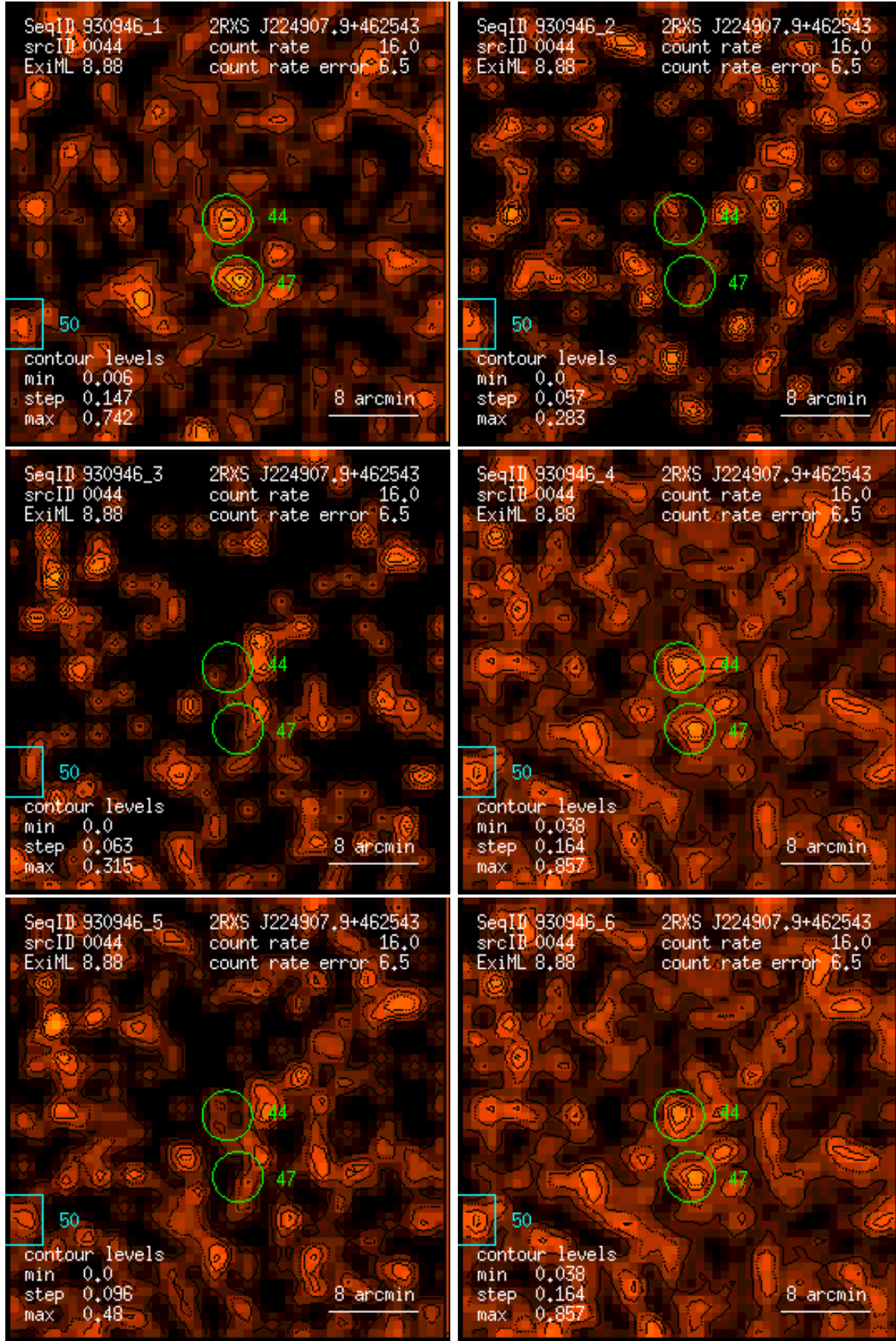
Figure 44: RASS 930946: detection 0044: band rate images, Gaussian filter: (1) PSPC channels 11 – 41, (2) 52 – 90, (3) 91 – 201, (4) 11 – 235, (5) 52 – 201, (6) 11 – 201. Broad band rates in counts/ks. Band rate contour levels in counts/ks/arcmin 2 .
